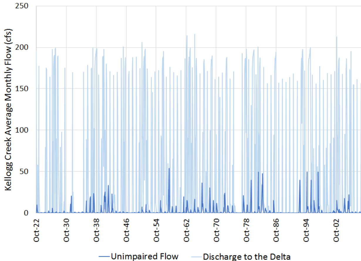
Figure A - 2 SacWAM Monthly Average Flow in Kellogg Creek
