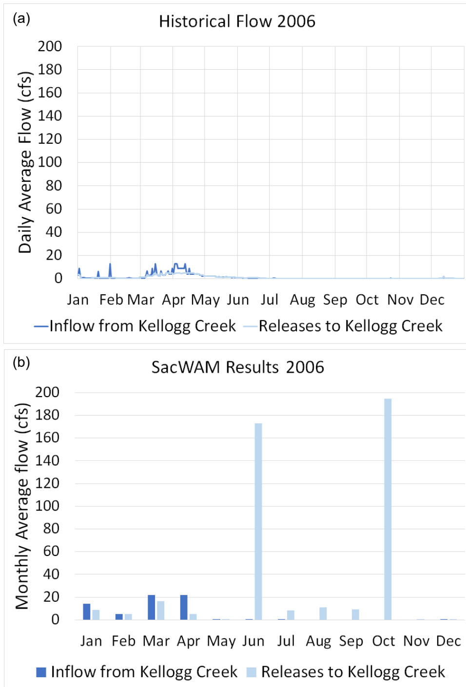
Figure A - 4 Inflow from Kellogg Creek and Releases to Kellogg Creek from Los Vaqueros Reservoir in 2006: (a) historical daily average flow and (b) SacWAM monthly average results
