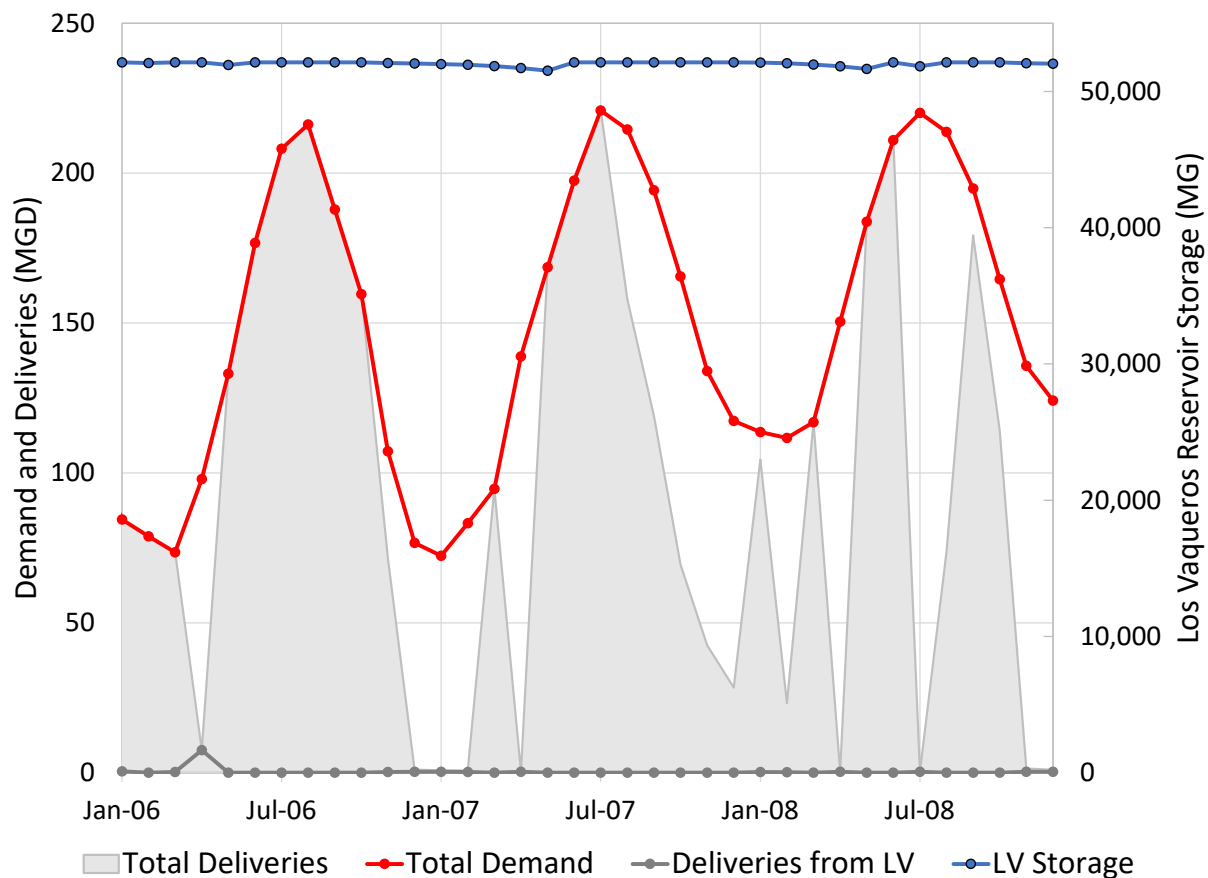
Figure A - 5 Total Demand and Deliveries to U_CCWD and Storage in Los Vaqueros Reservoir
