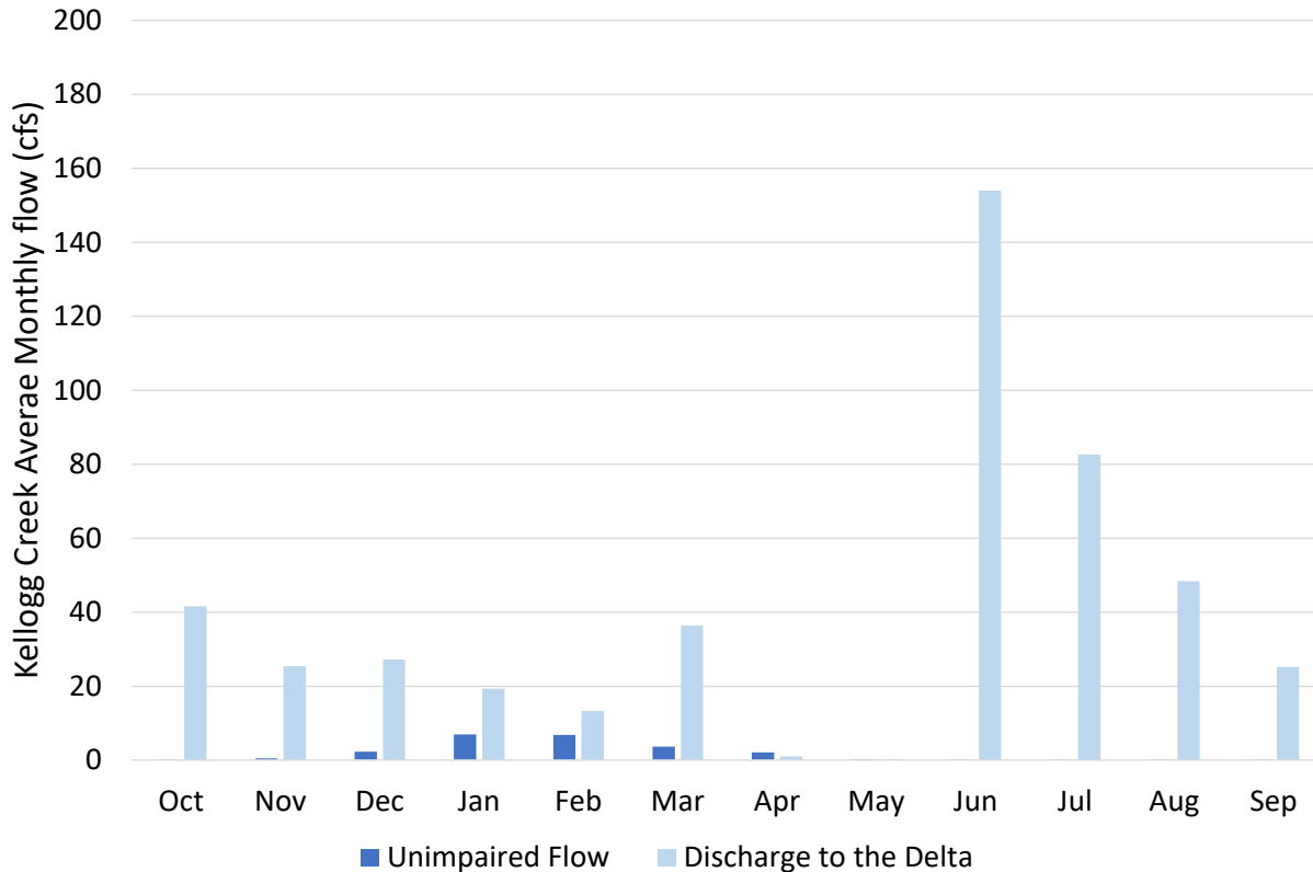
Figure A - 3 SacWAM Long-term (1922-2009) Average Monthly Flow in Kellogg Creek
