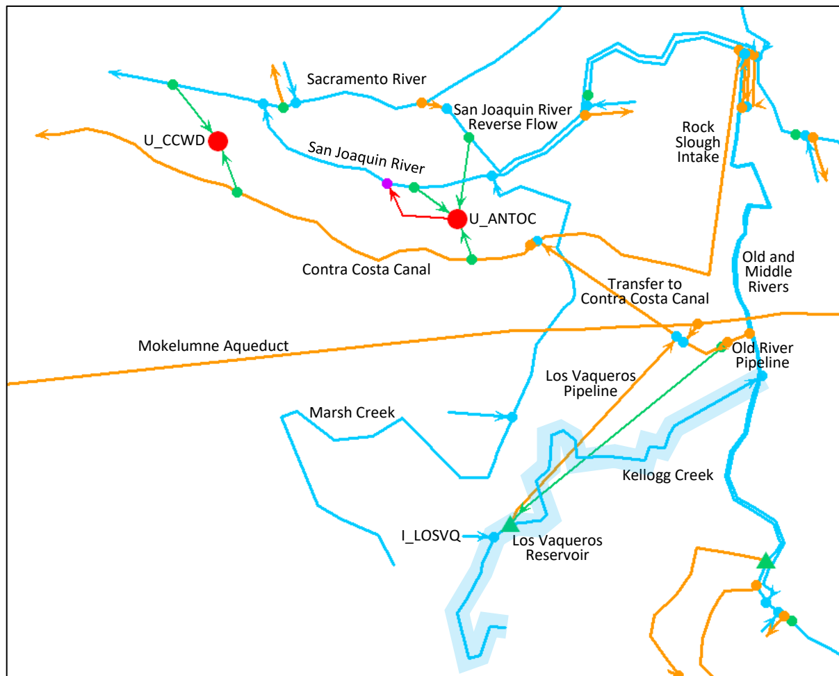
Figure A - 1 SacWAM schematic of Kellogg Creek (highlighted) and surrounding area
