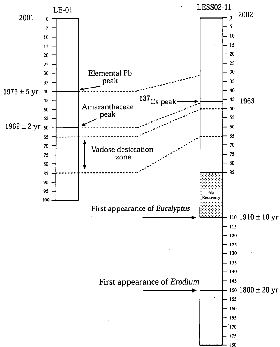
Figure 7. Chronological markers for LE-01 and LESS02-11. Dashed lines indicate probable depth equivalents between the two cores based on water content (see Fig. 2).
