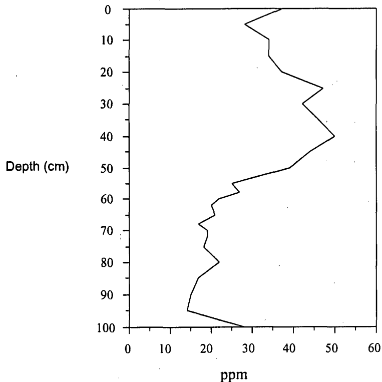
Figure 4. Lead concentration in LE-01.
