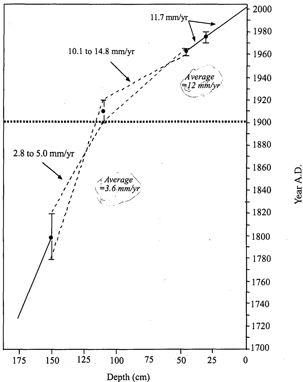
Figure 9. Age Depth Curve with sedimentation rates for core LESS02-11. Solid line is the linear age-depth extrapolation to core bottom. The bottom of the core is approximately 1730. Note the difference in sedimentation rates between the pre-20th century and the 20th century period.
