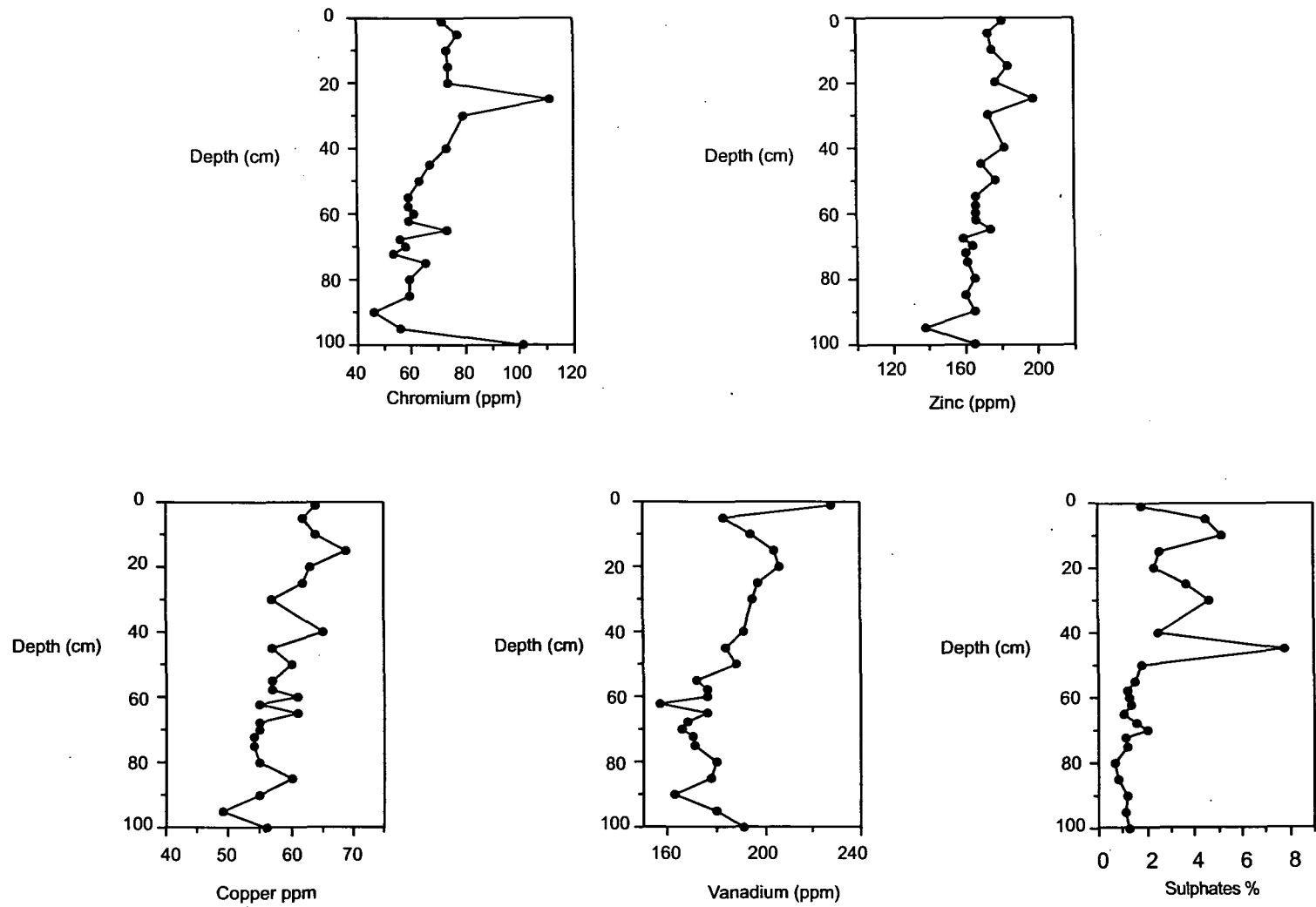
Figure 5. Concentrations of chromium, zinc, vanadium, copper and sulfates in LE-01.
