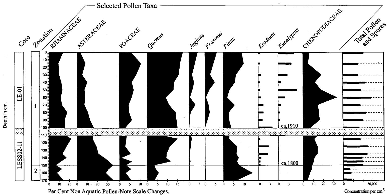
Figure 3. Pollen diagram showing pollen frequencies for core LE-01 and the lower section of LESS02-11.
