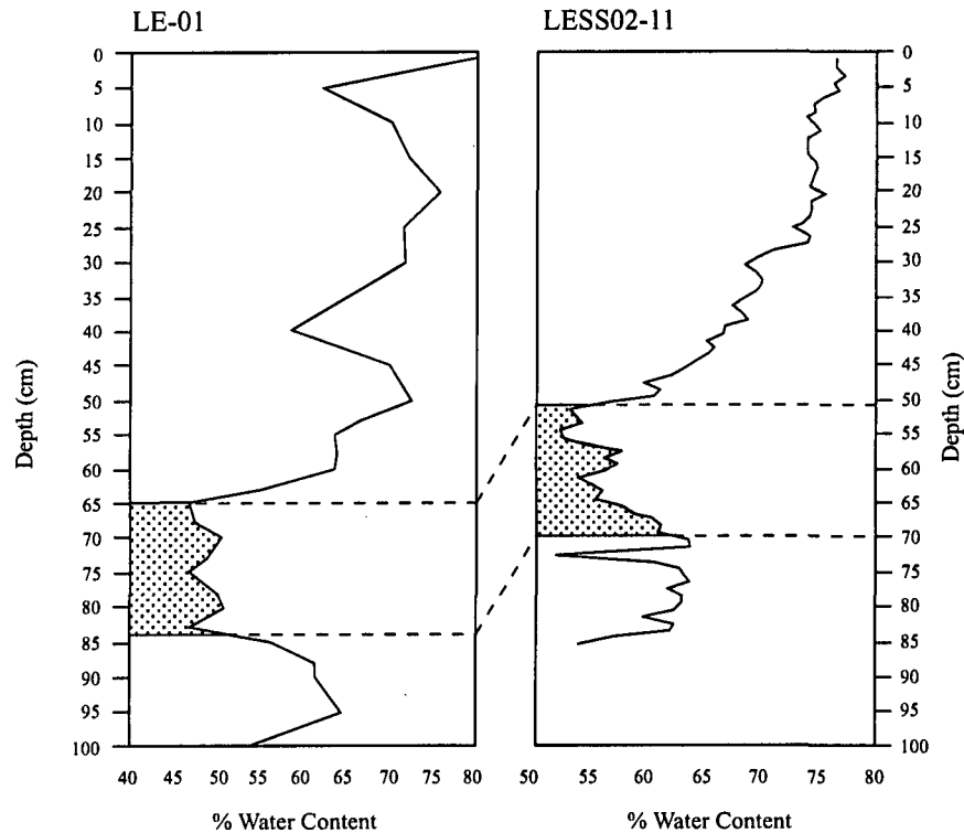
Figure 2. Percent total water content for core LE-01 and LESS02-11. Vadose desiccation zone shown by shaded area
