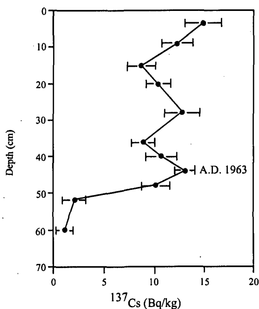
Figure 5. Cesium-137 profile for core LESS02-11.
