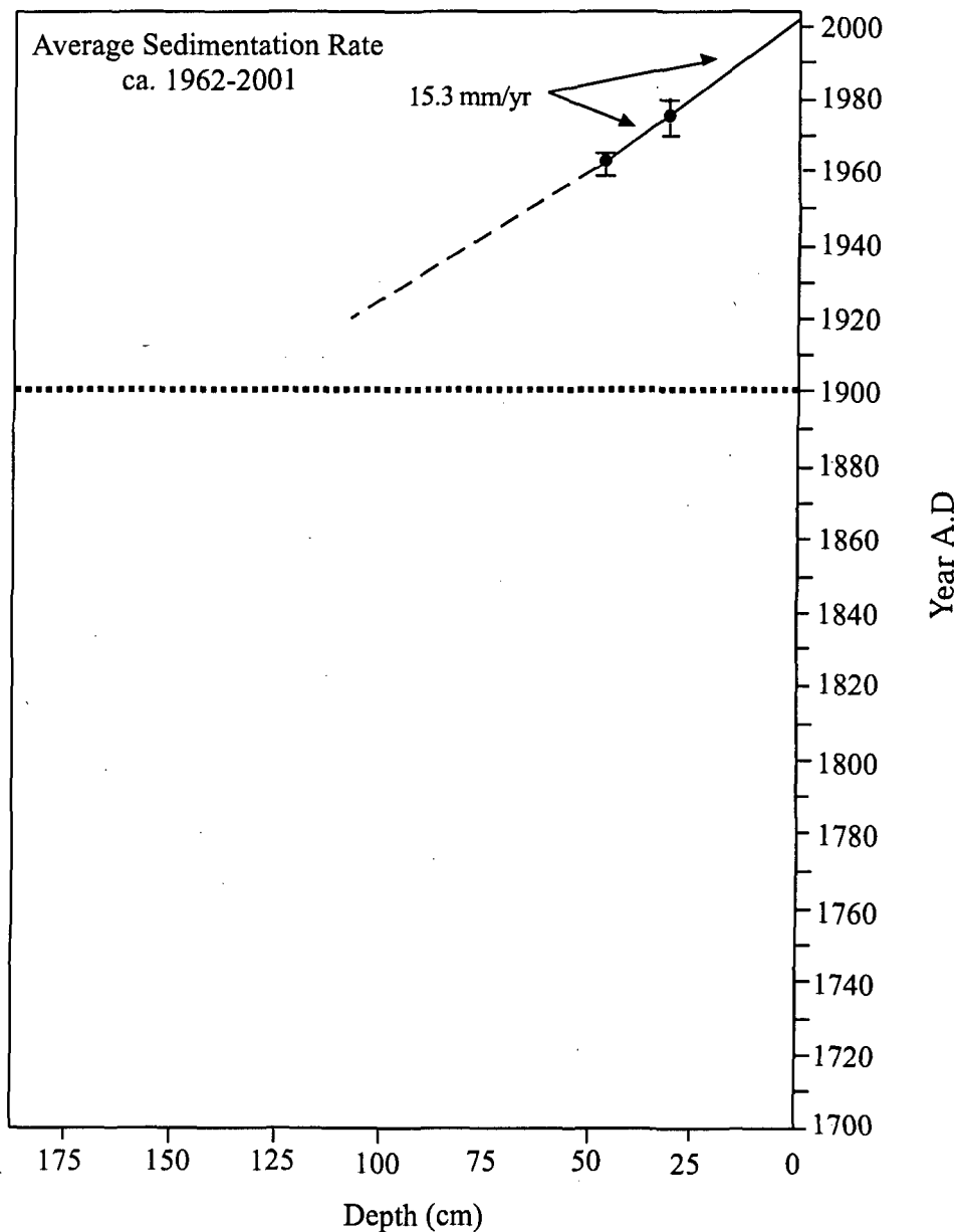
Figure 8. Age Depth Curve with sedimentation rates for core LE-01. Dashed line is the linear age-depth extrapolation to the core bottom. If the extrapolation is correct the bottom of the core dates to approximately 1920.
