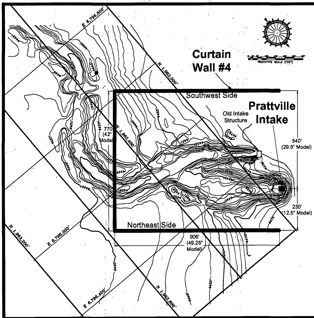
Figure 7-7. Layout and dimensions of Curtain No. 4
