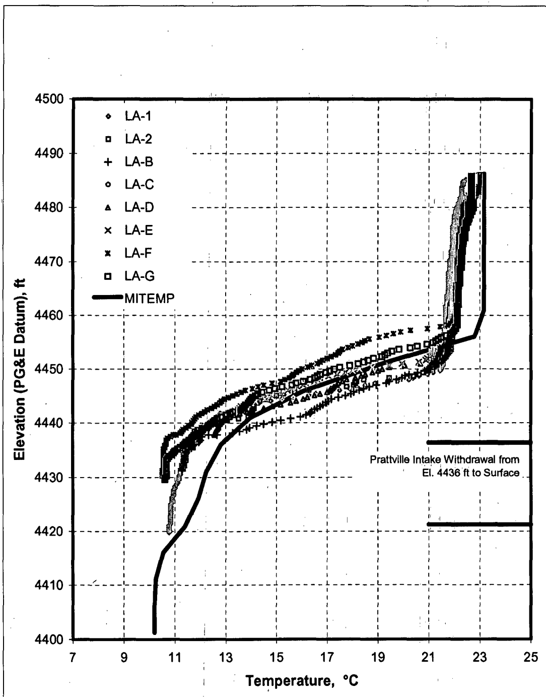
Figure 2-5 continued. Water temperature profiles measured in Lake Almanor: (c) on August 17, 2000 (data provided by PG&E).
