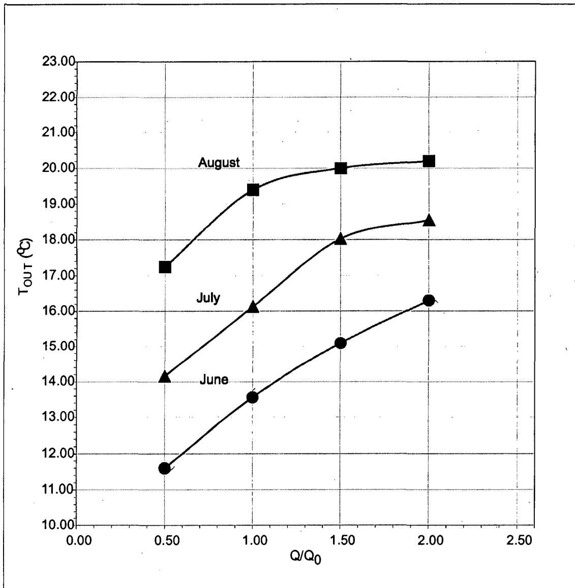
Figure 6-9. Variation of outflow temperature, T_{out} , with Q/Q_0 for the Bay testboxes subject to June, July, and August conditions.
