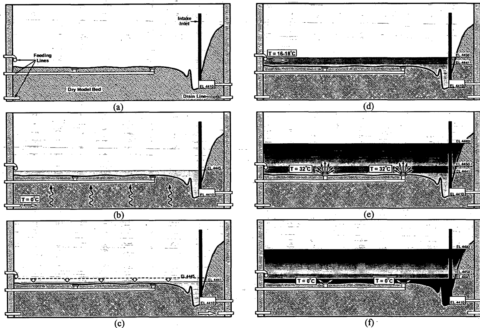
Figure 3-11. Typical sequence for attaining prescribed water temperature profiles in the model: (a) dry bed; (b) cold-water feeding for bed cooling; (c) removal of excess water; (d) buffer-layer feeding; (e) warm-layer feeding; (f) final cold-layer feeding.
