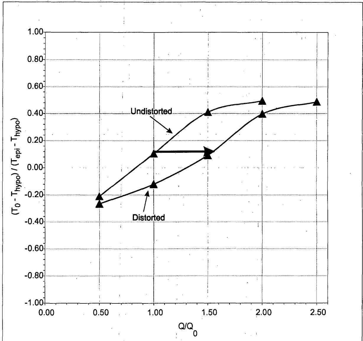
Figure 6-4. Normalized results from Bay testboxes; July condition.
