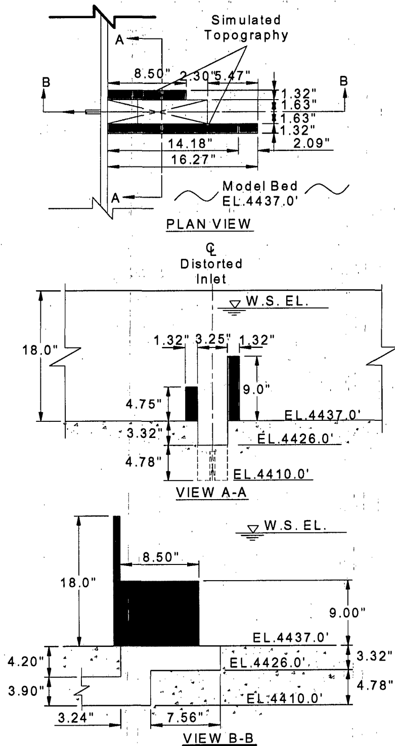
Figure 4-10. Layout and dimensions of the distorted Open testbox.
