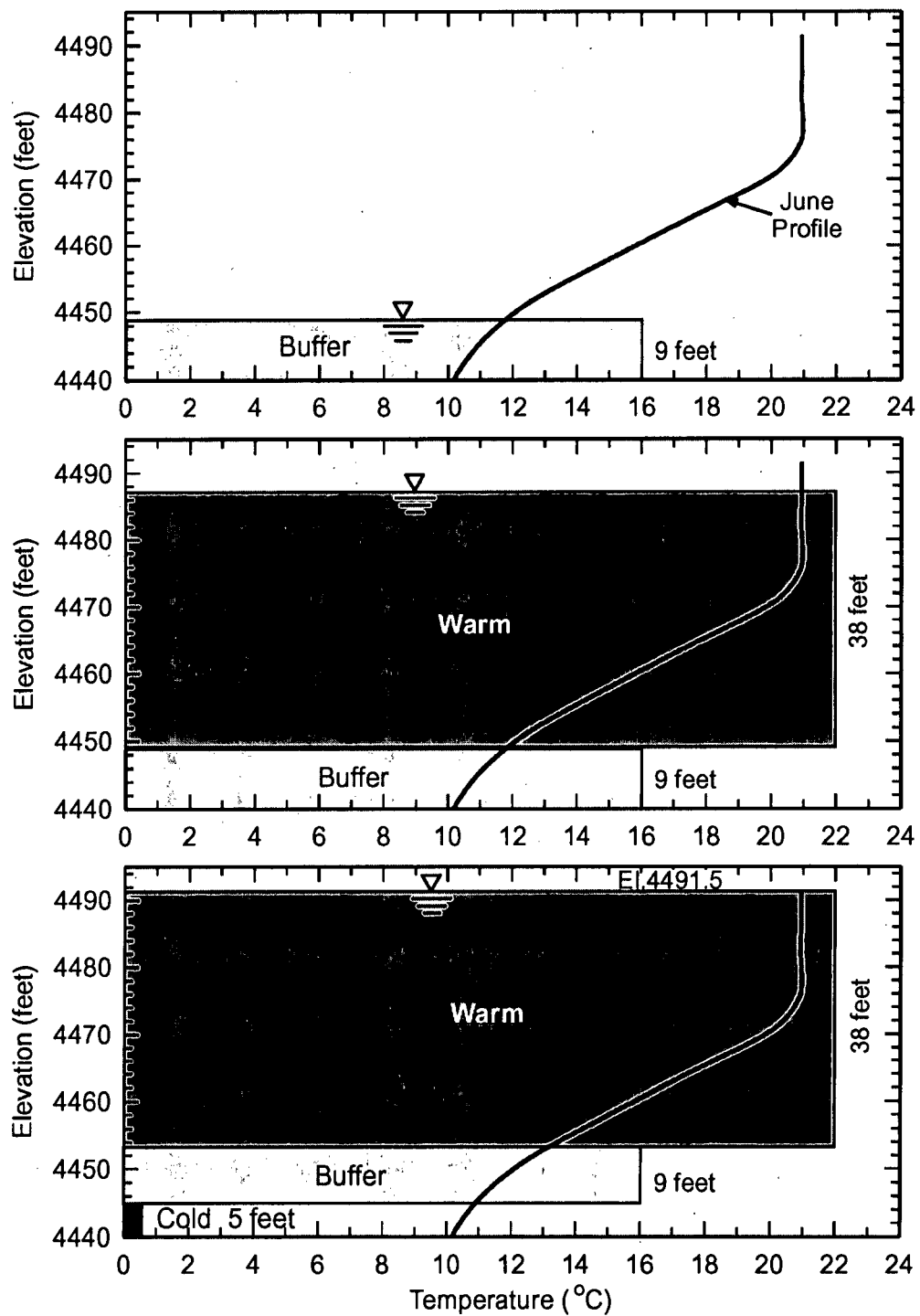
Figure 3.12. Development of June condition temperature profile.
