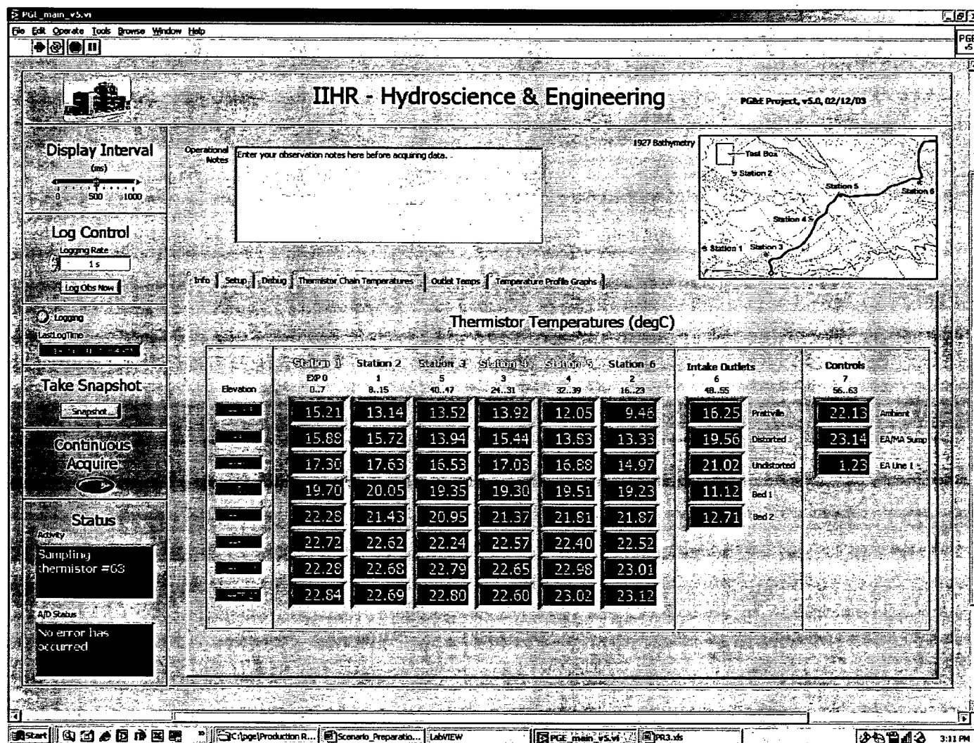
Figure 3-18. Interface for thermistor-chain temperatures.
