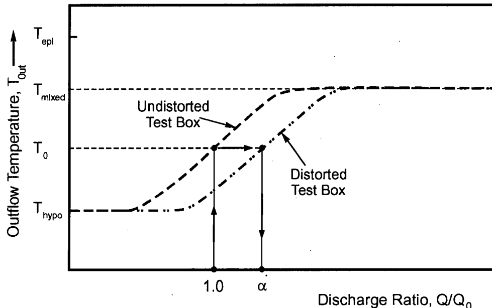
Figure 3. Conceptual relationship between outflow temperature and discharge ratio in the distorted and undistorted testboxes, indicating the discharge-calibration factor \alpha .
