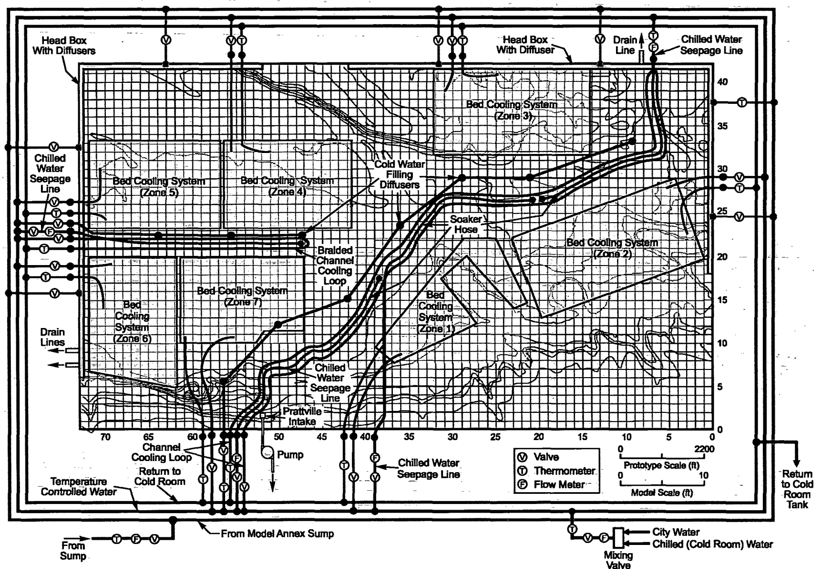
Figure 3-9. Layout of the water lines in the hydraulic model.
