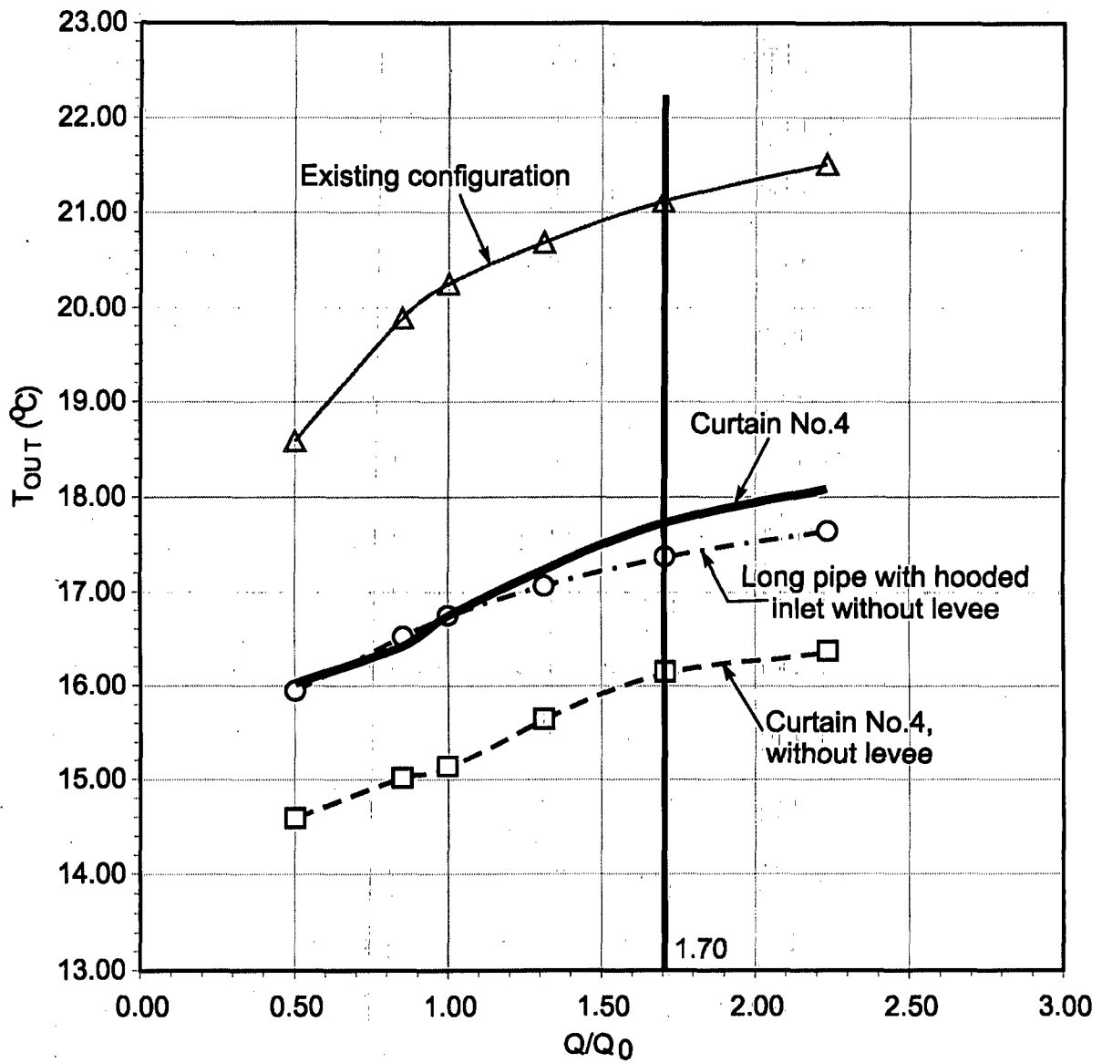
Figure 7-35. Comparison of the performances of LPHI with levees removed and Curtain No. 4 (with and without levees); August condition.
