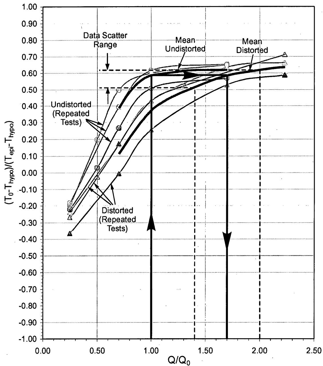
Figure 6-5. Normalized results from the Open testboxes; July condition.
