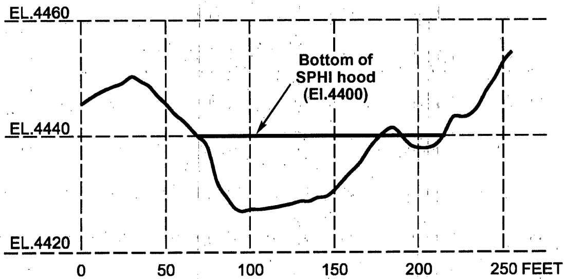
Figure 7-27. Elevation view of the cross-section through the hood and the incised channel (prototype dimensions) for the modeled SPHI.
