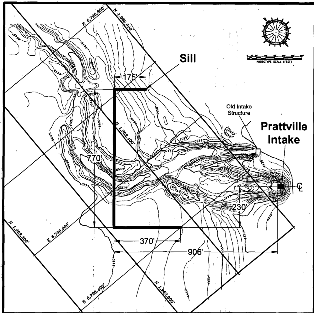
Figure 7-37. Layout of the bottom sill. The sill crest is at 4450 ft.
