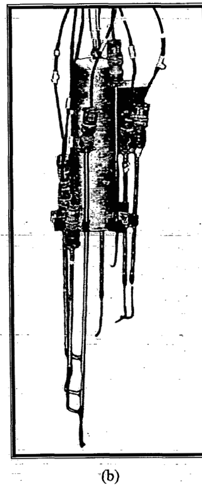
Figure 3-17. Thermistor chain arrangement: (a) schematic; (b) photograph.
