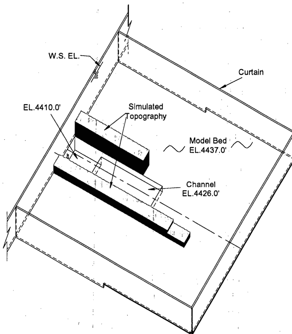
Figure 8-5. Perspective view of the undistorted Open testbox with curtain.
