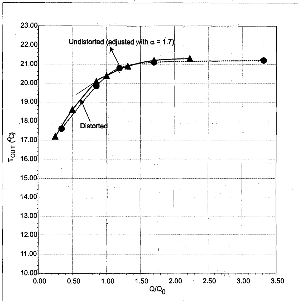
Figure 6-10. Comparison of results from the distorted Open testbox and from the undistorted Open testbox (adjusted with the calibration factor \alpha = 1.7 ); August condition.
