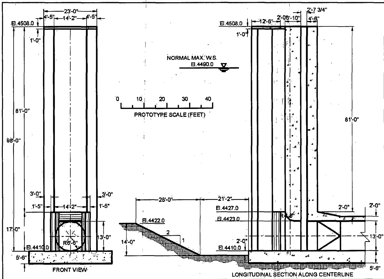
Figure 2-3. Layout and dimensions of the Prattville Intake.
