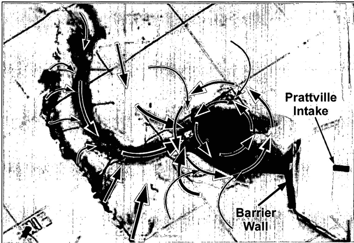
Figure 7-30. Visualization of the flow approaching the SPHI. The arrows indicate flow paths produced by the short pipe with hooded inlet.
