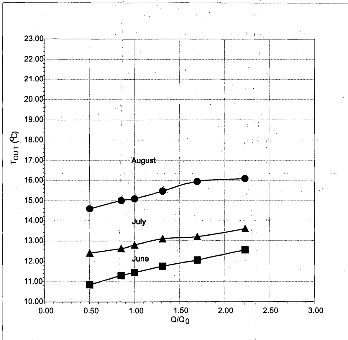
Figure 7-20. Outflow temperature obtained with Curtain No. 4 and levees removed, for the June, July, and August conditions.
