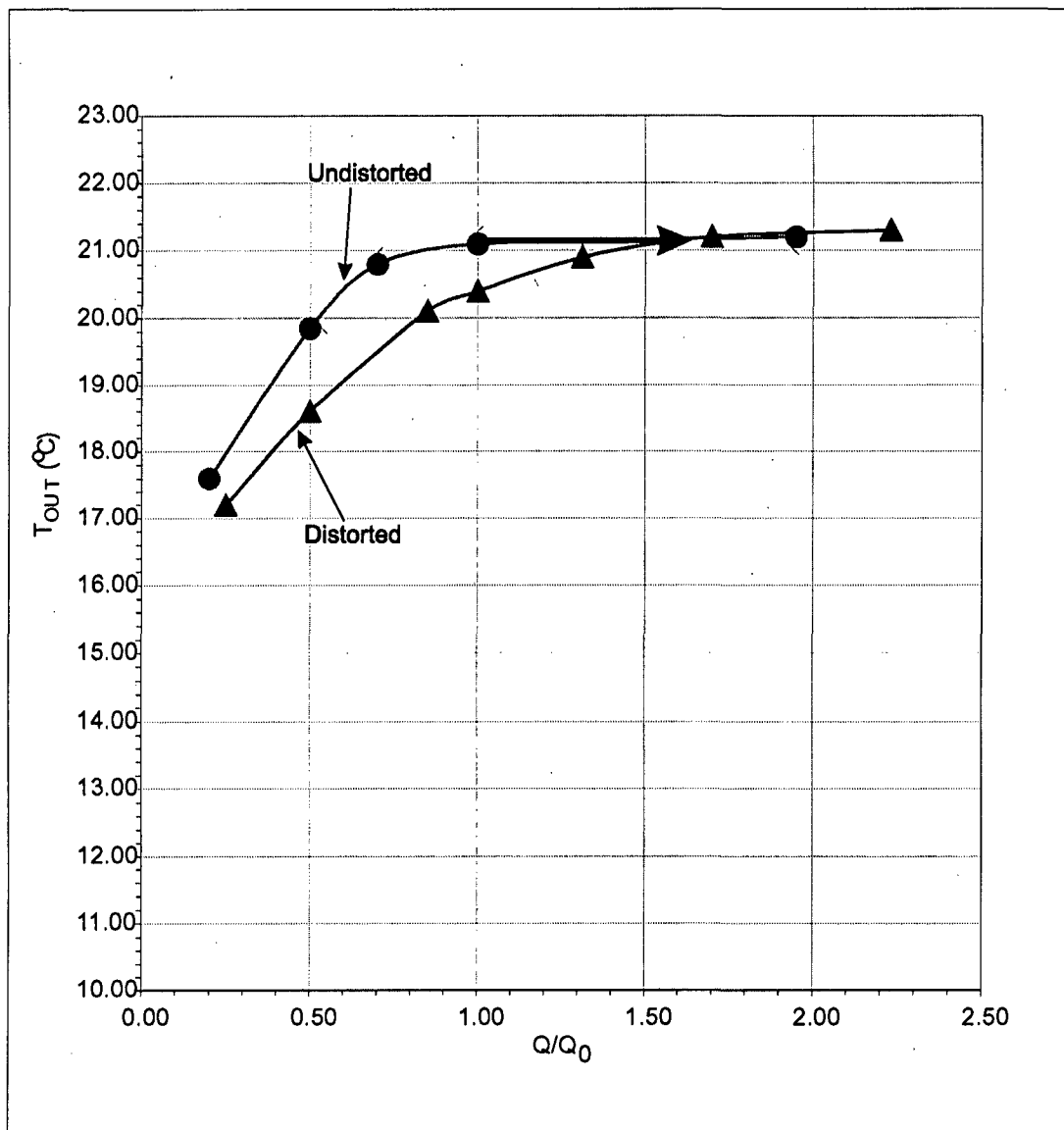
Figure 6-7. Results from Open testboxes; August condition (no curtain).
