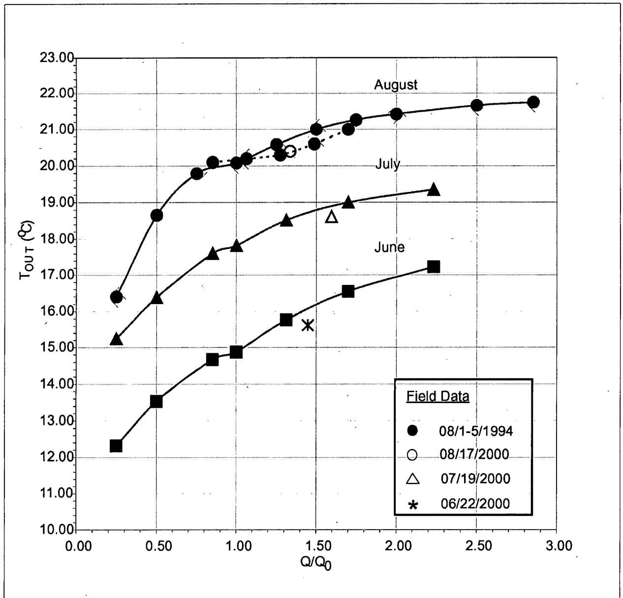
Figure 8-1. Validation of the hydraulic model results with field data. The field data are adjusted by factor \alpha = 1.7 applied to Q/Q_0 .
