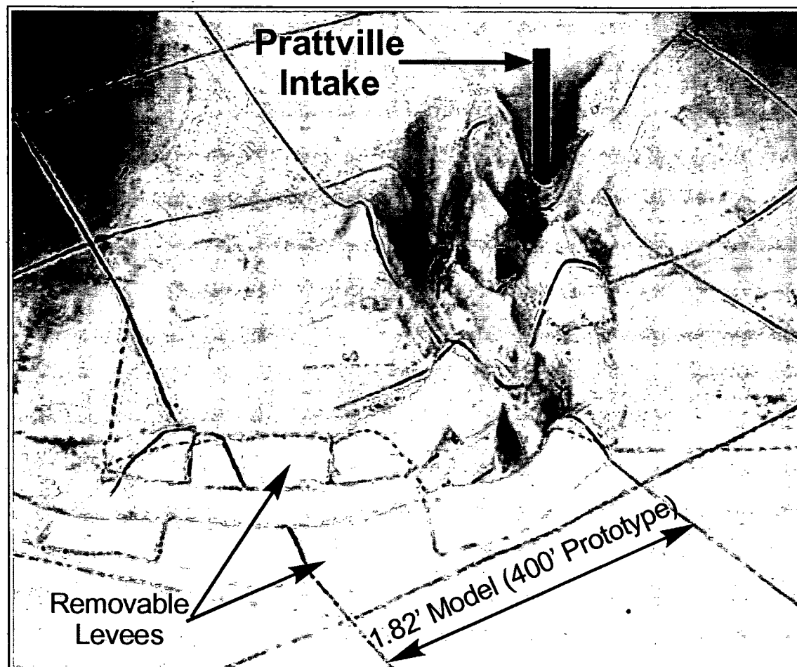
Figure 3-8. Model bed topography near Prattville Intake. Grid on bottom represents a 400 ft by 400 ft prototype grid.
