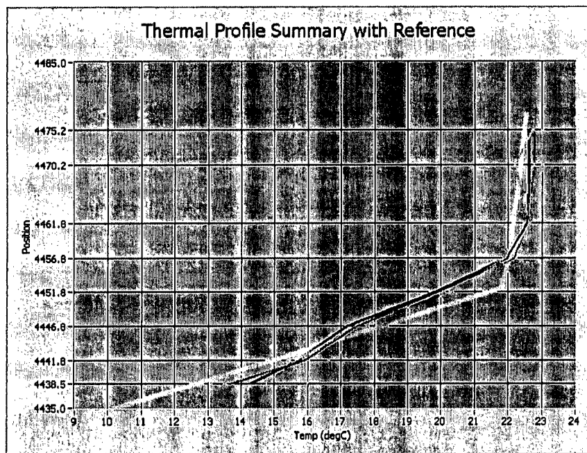
Figure 3-13 continued. (c) At the end of cold-water feeding (final profile).
