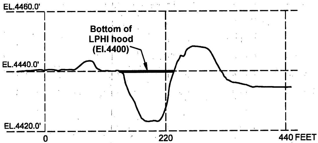
Figure 7-32. Elevation view of the cross-section through the hood and the incised channel (prototype dimensions) for the modeled LPHI.
