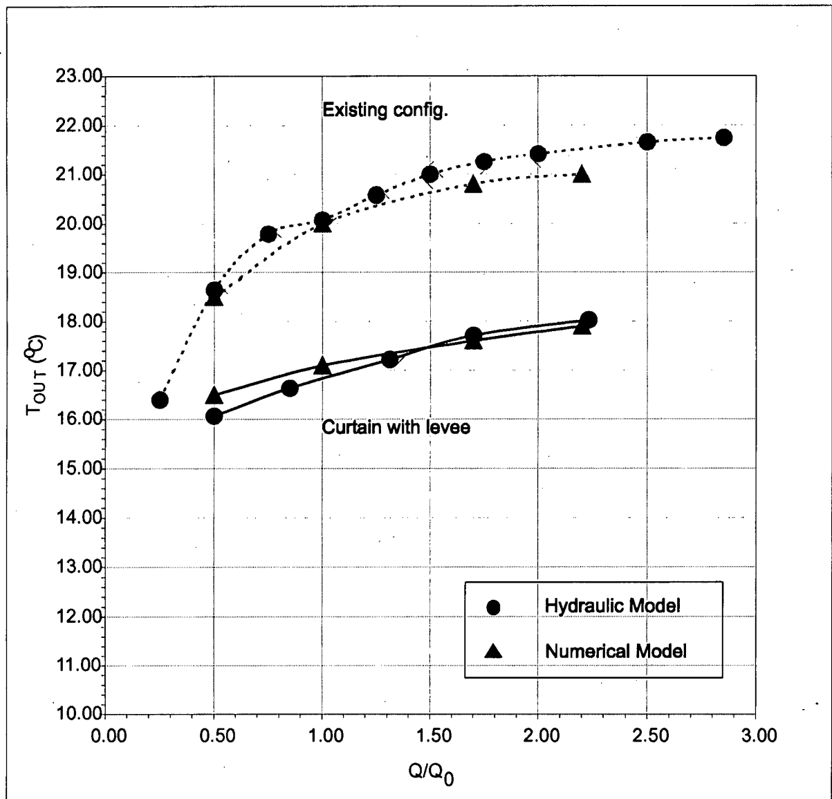
Figure 8-11. Comparison of numerical-model and hydraulic-model results for vertically distorted representation of Prattville Intake. The results are for the Intake with and without Curtain No. 4 for August condition. Note that the levees were not removed.
