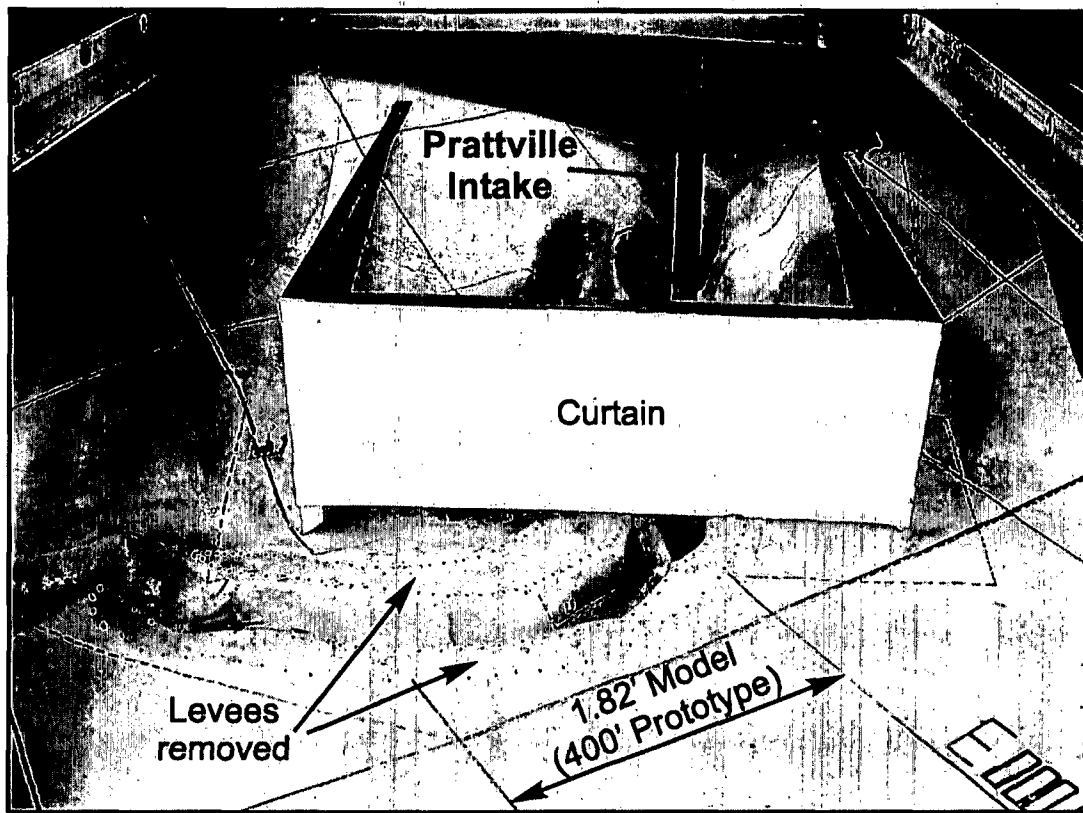
Figure 4. Prattville Intake surrounded by the recommended skimming curtain, and the levees removed in front of the curtain.
