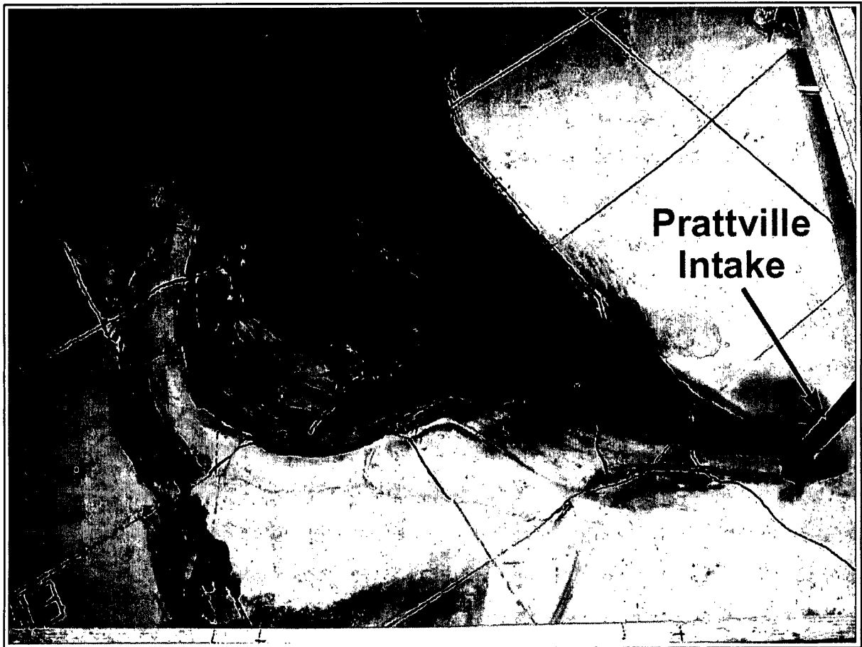
Figure 7-5. Visualization of flow to Prattville Intake ( Q/Q_0 = 1.7 , August condition). (a) Visualization with dye. Dye is released into approach flow outside the incised channel, blue dye into colder bottom layer and red dye into the warmer surface layer. The intake withdraws predominantly warm surface water.
