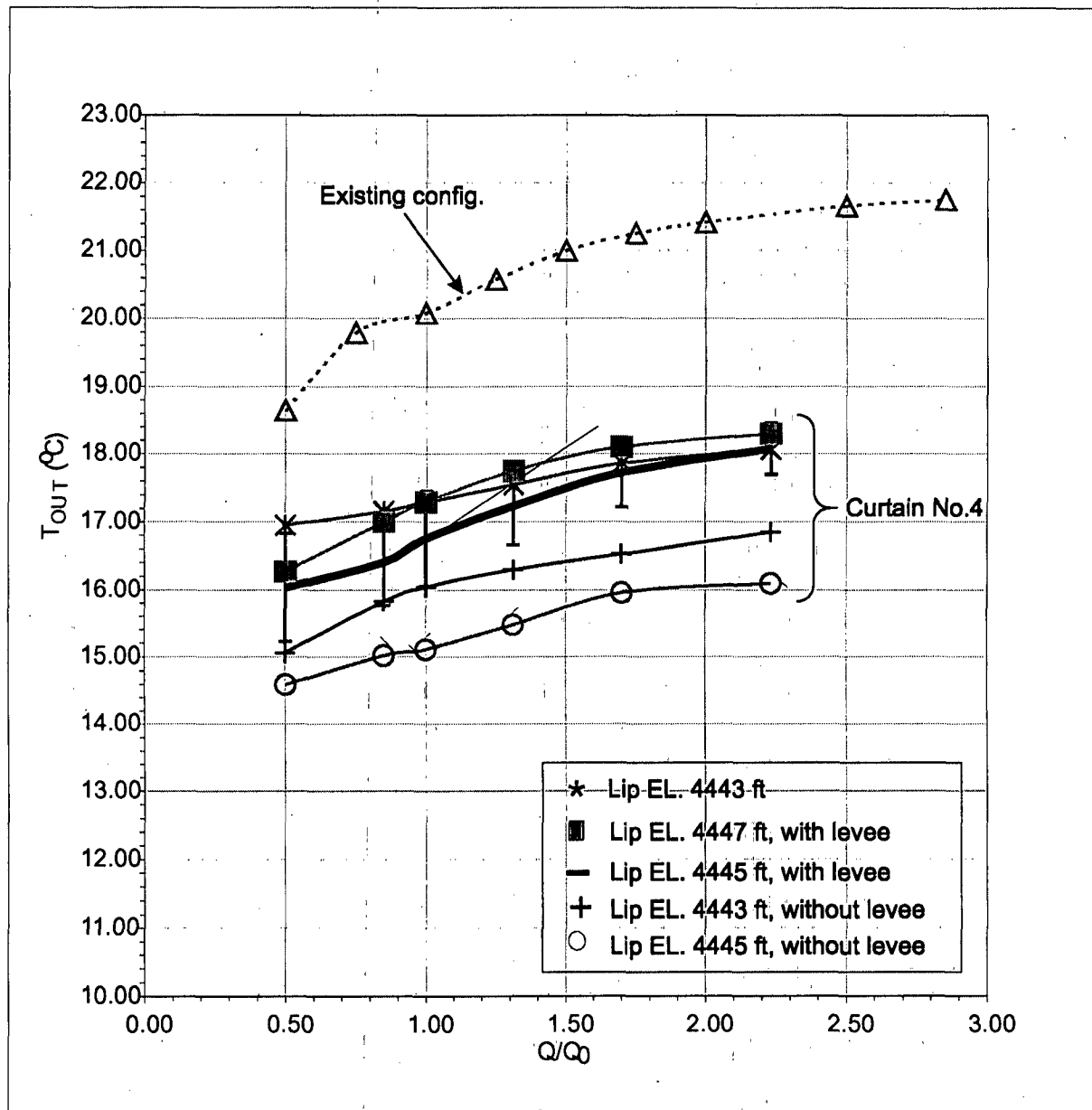
Figure 8-2. Sensitivity of Curtain No. 4 with variation of lip elevation (tests conducted for August condition).
