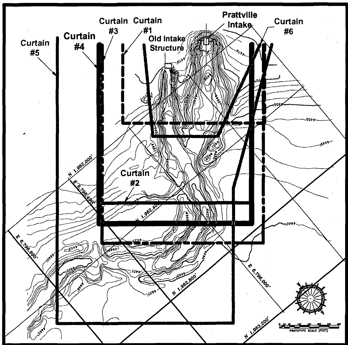
Figure 7-6. Layouts of the curtains tested. Curtain No. 4 was selected for further testing.
