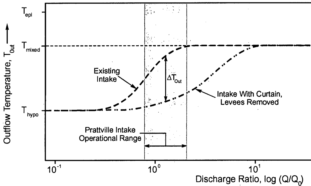
Figure 5. Conceptual illustration of the effect of the skimming curtain on the temperature of outflow released from Prattville Intake.
