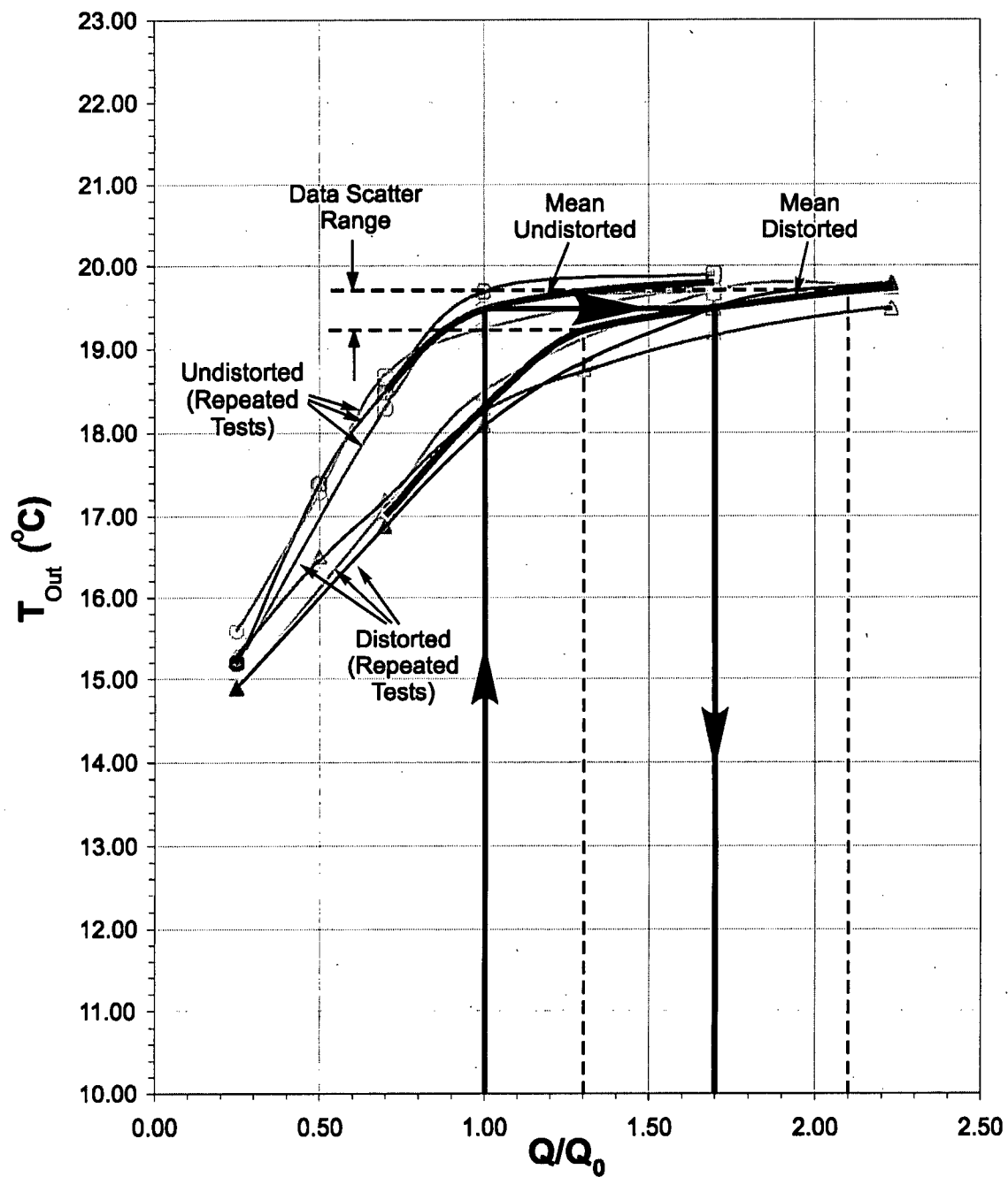
Figure 6-3. Results from Open testboxes; July condition.
