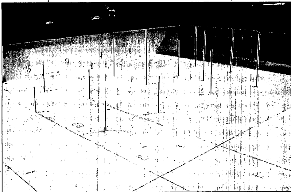
Figure A.3. Grade pins used for setting model bathymetry
