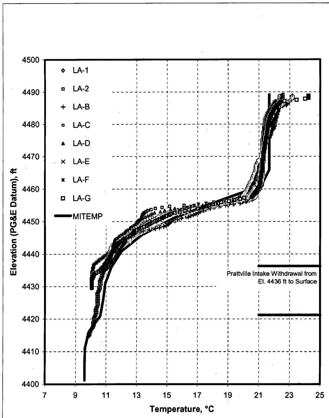
Figure 2-5 continued. Water temperature profiles measured in Lake Almanor: (b) on July 22, 2000 (data Provided by PG&E).
