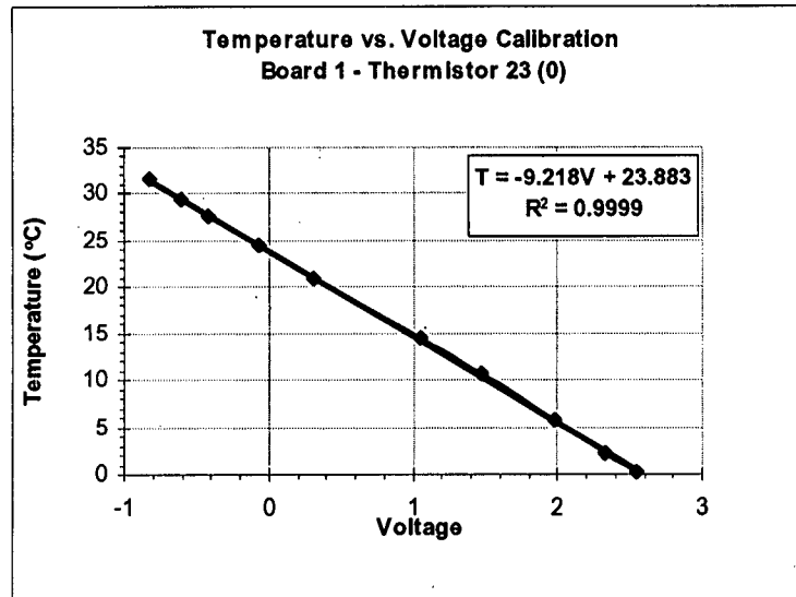
Figure 4-2. Example of thermistor calibration curve.
