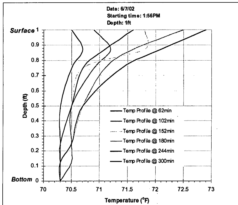
Figure 4-3. Temperature variation over time for a uniform body of water placed in the test tank.
