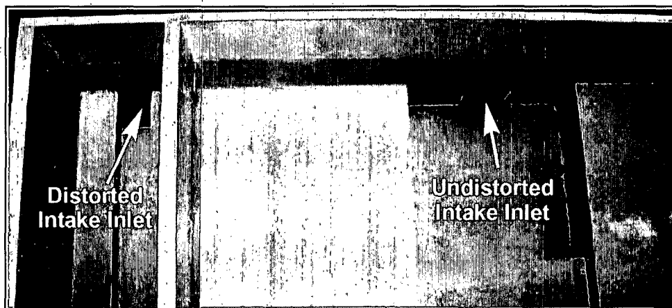
Figure 4-6. Photographs of the distorted and undistorted Bay testboxes. For each testbox the simplified intake was located in a recess below the replicated lakebed. The intake's invert was located at the actual elevation for Prattville Intake. The testboxes included a compound channel that approximately replicated the man-made channel excavated along the bed of Lake Almanor.
