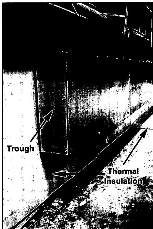
Figure A.2. Detail of insulation positioning (1 inch-thick insulation on wall; 1.5 inch-thick insulation on the model floor)
