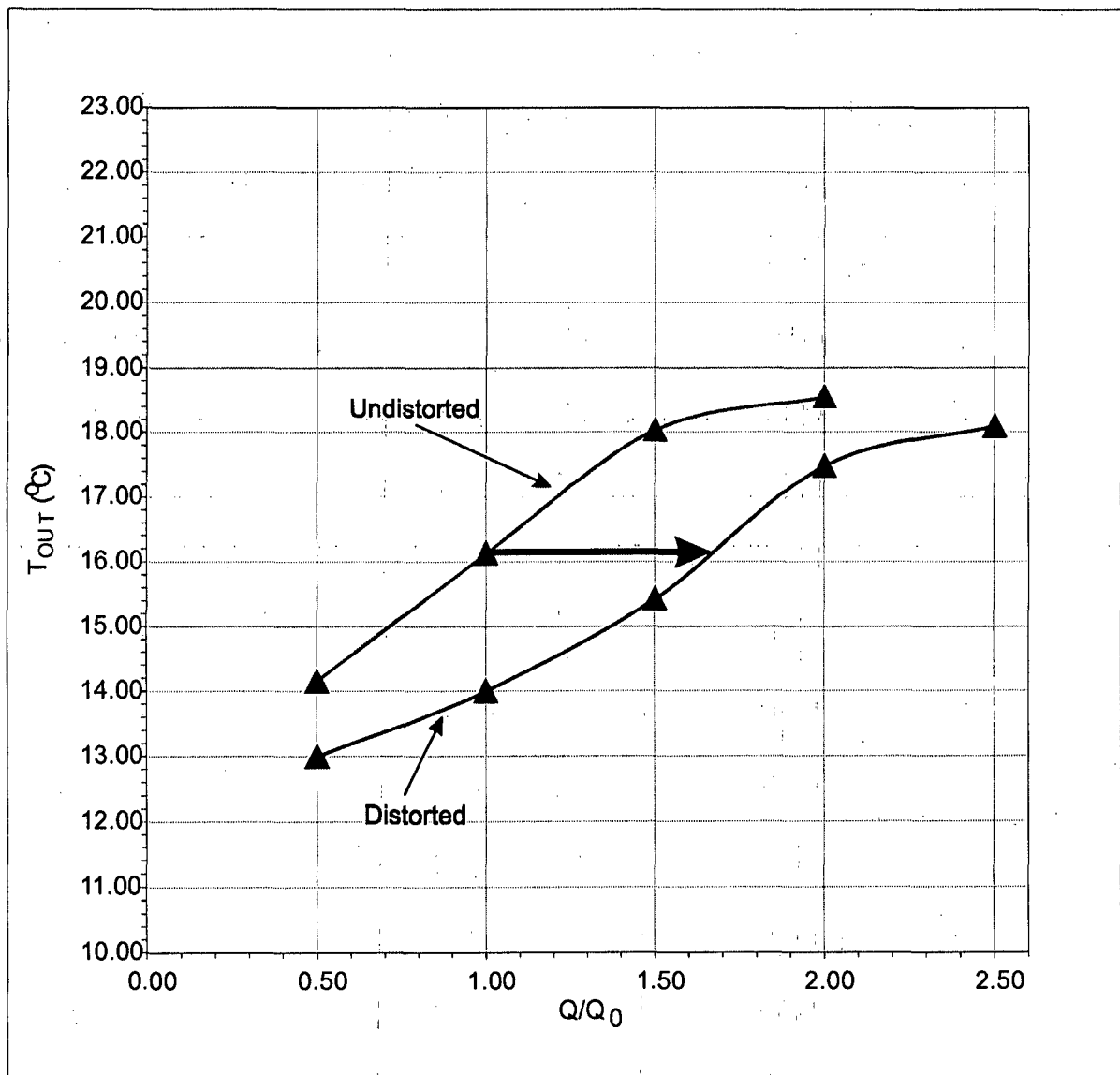
Figure 6-2. Results from Bay testboxes: July condition.
