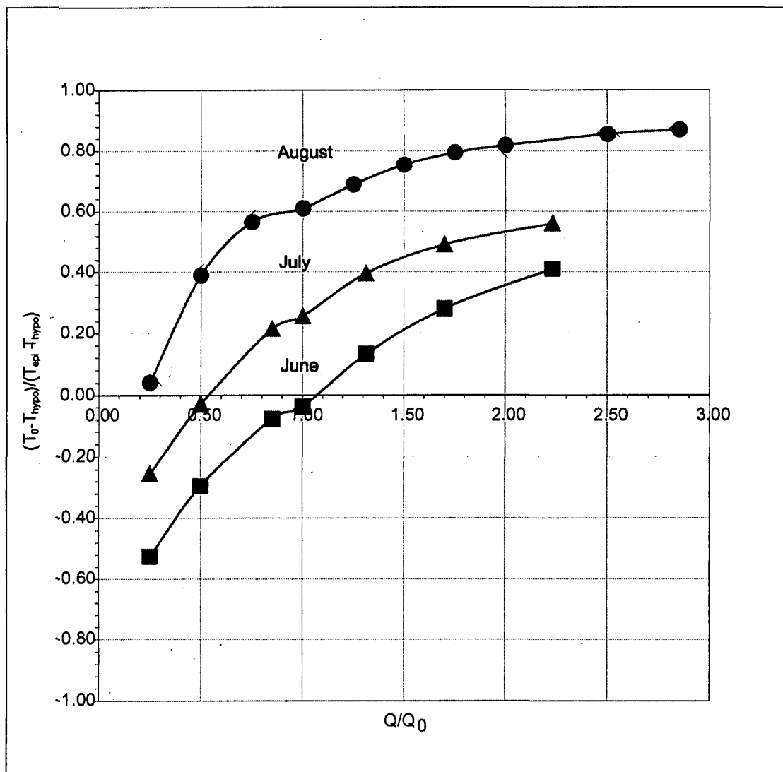
Figure 7-3. Normalized outflow temperature obtained with the hydraulic model for June, July and August.
