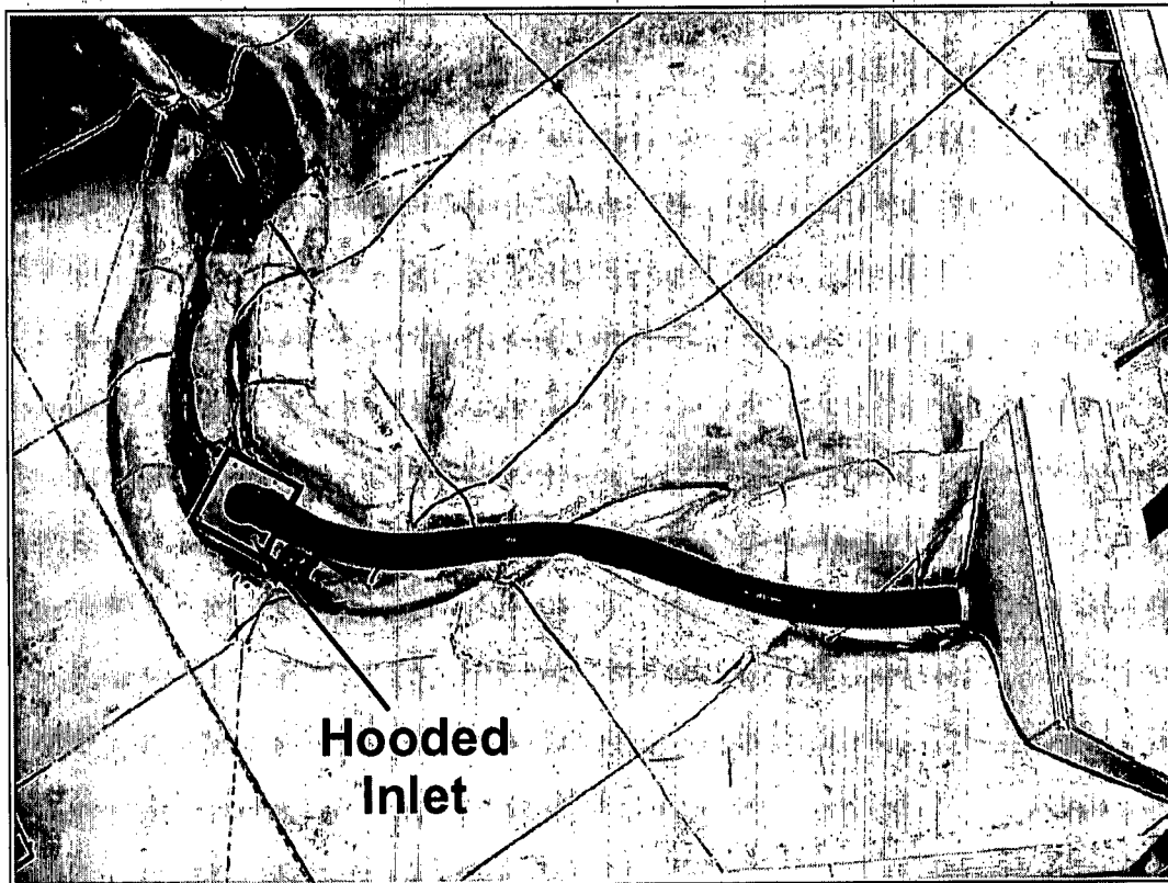
Figure 7-33. View of the LPHI in the model.
