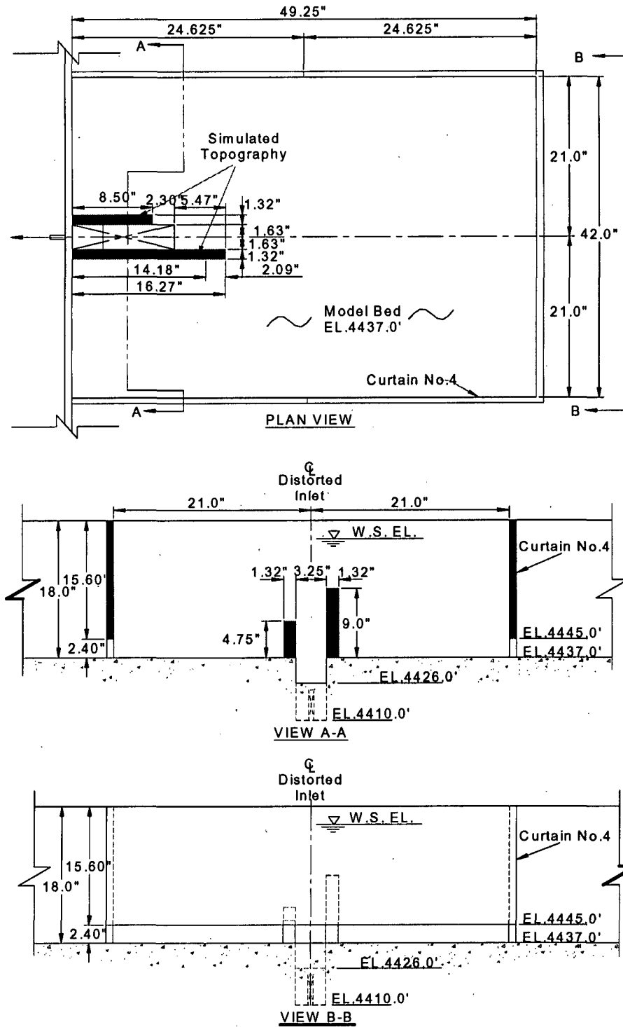
Figure 8-8. Layout and dimensions of Curtain No. 4 placed around the distorted Open testbox.
