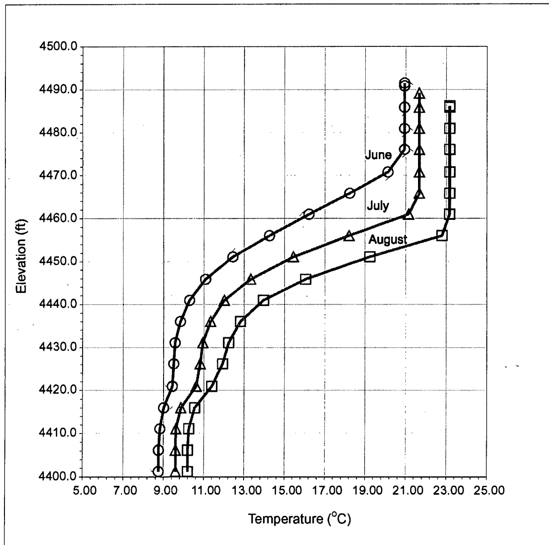
Figure 2-6. Average profiles of water temperature in Lake Almanor for June, July, and August 2000.
