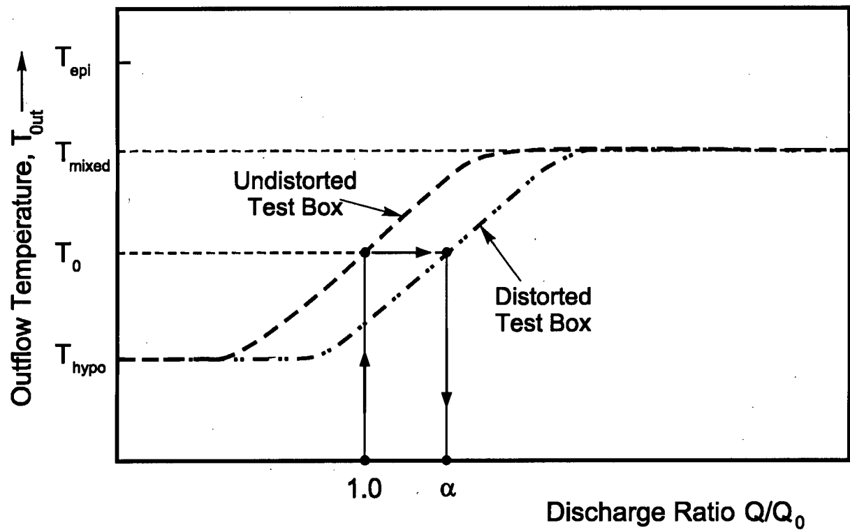
Figure 6-1. General relationship between the outflow temperature T_{out} and discharge ratio Q/Q_0 for the distorted and undistorted testboxes.
