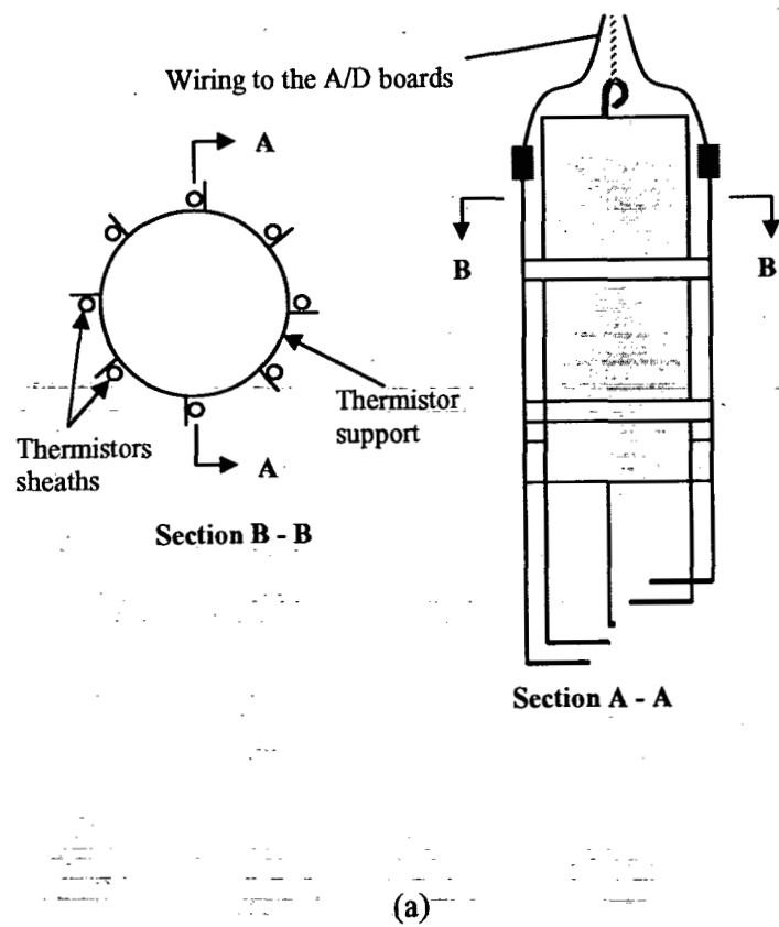
Figure 3-17. Thermistor chain arrangement: (a) schematic; (b) photograph.
