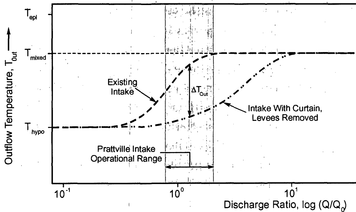
Figure 7-13. Conceptual trends showing the reduction in outflow temperature when the intake is fitted with a curtain. At very low rates of outflow, only cold water is withdrawn. At higher flow rates, the curtain's effectiveness decreases because fully mixed water passes beneath the curtain.
