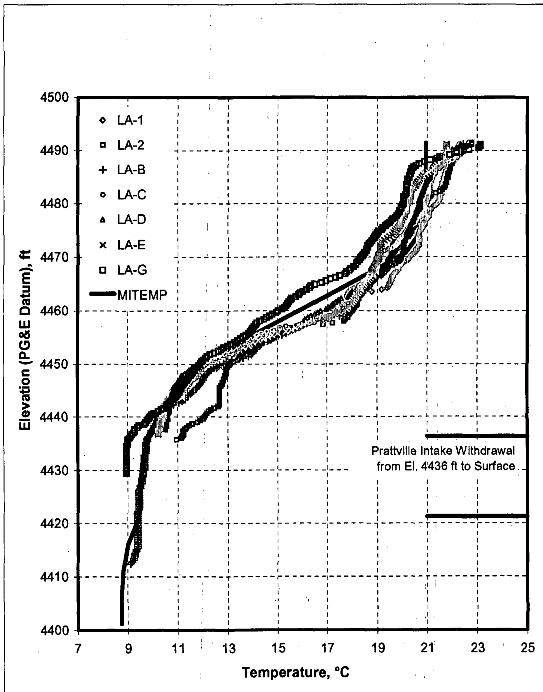
Figure 2-5. Water temperature profiles measured in Lake Almanor: (a) on June 20, 2000 (data provided by PG&E).
