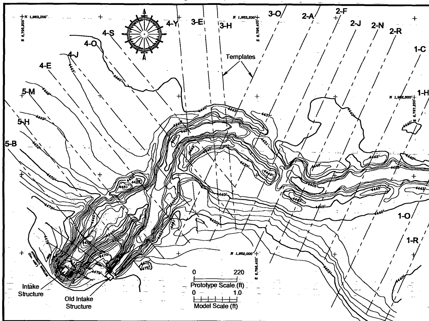
Figure 3-7. Bathymetry templates selected for constructing the area near the Intake.
