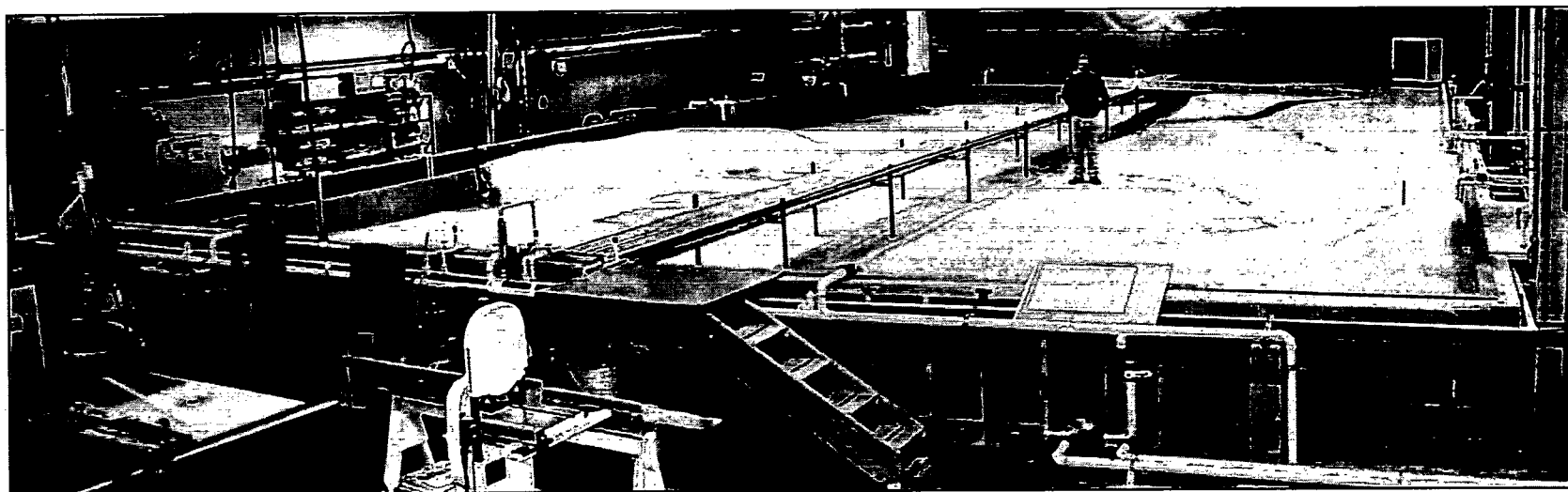
Figure 3-3. View of hydraulic model.
