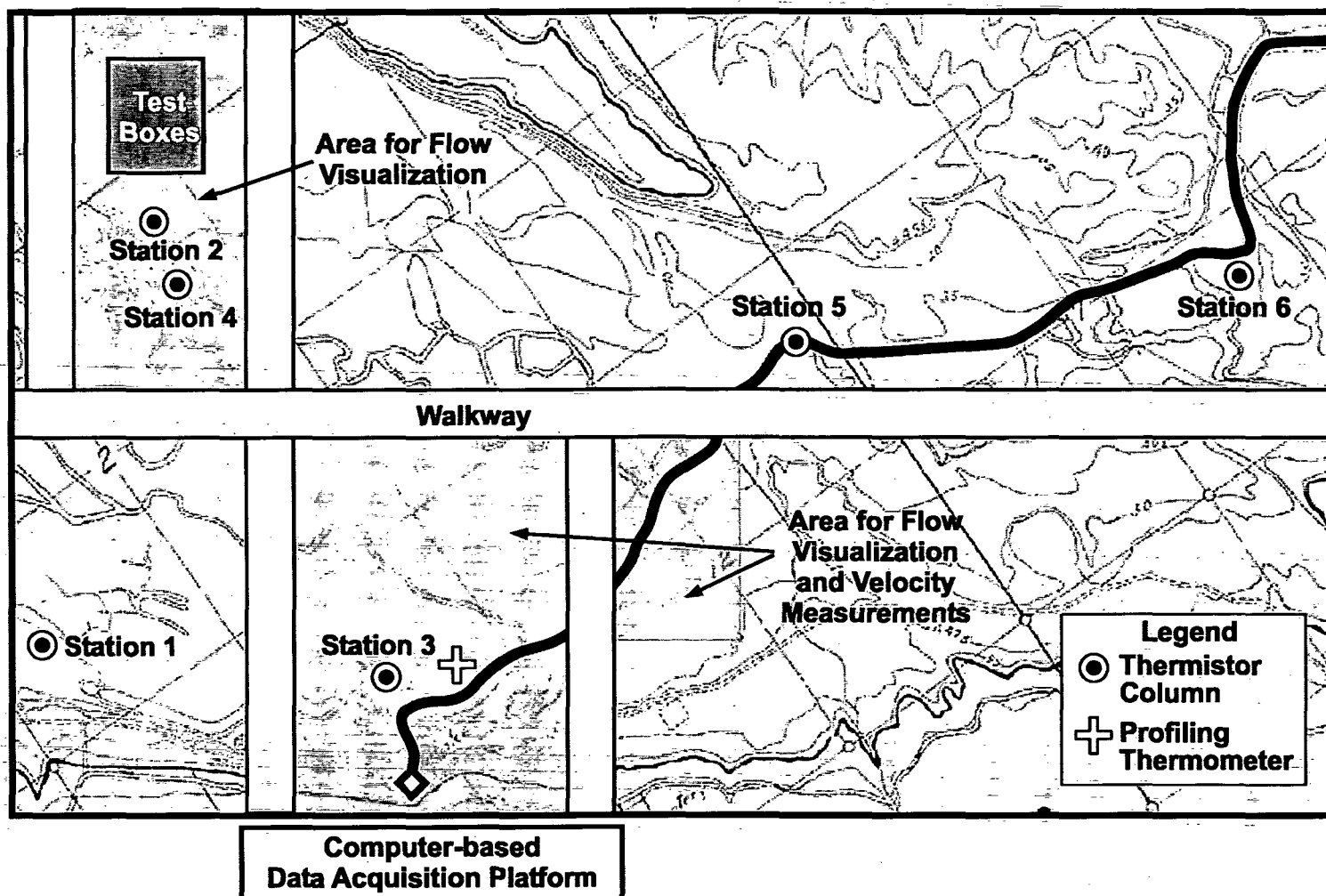
Figure 3-15. Layout of measurement system.
