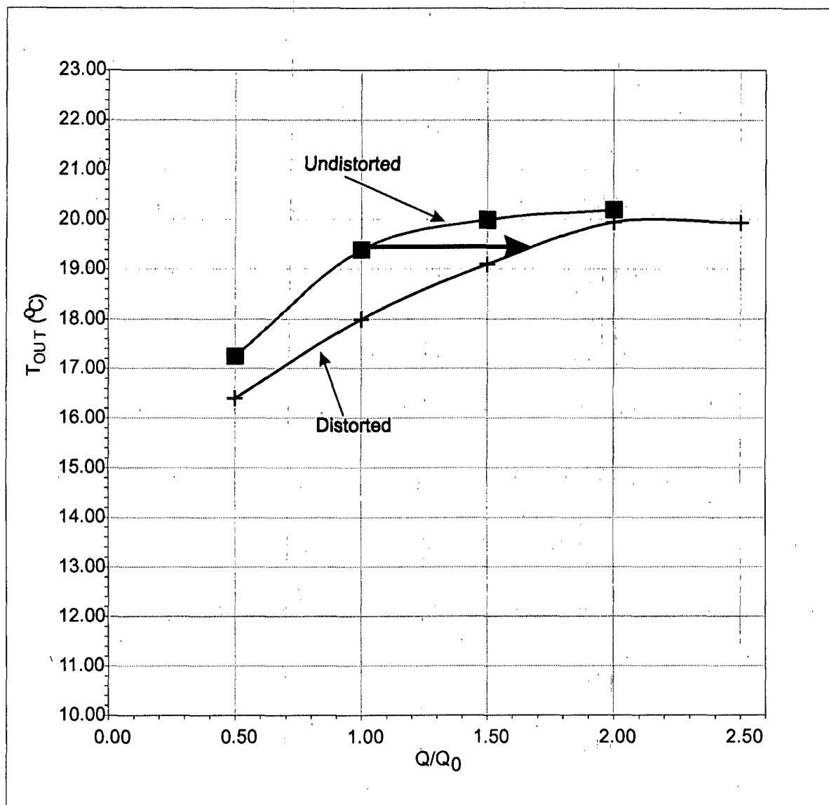
Figure 6-6. Results from Bay testboxes; August condition (no curtain).
