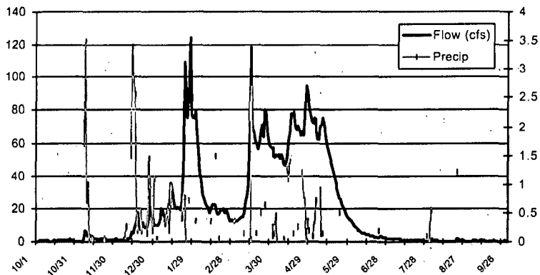
Last Chance Creek at Doyle Crossing Daily Average Flow and Precipitation at Genesee - Water Year 2003
