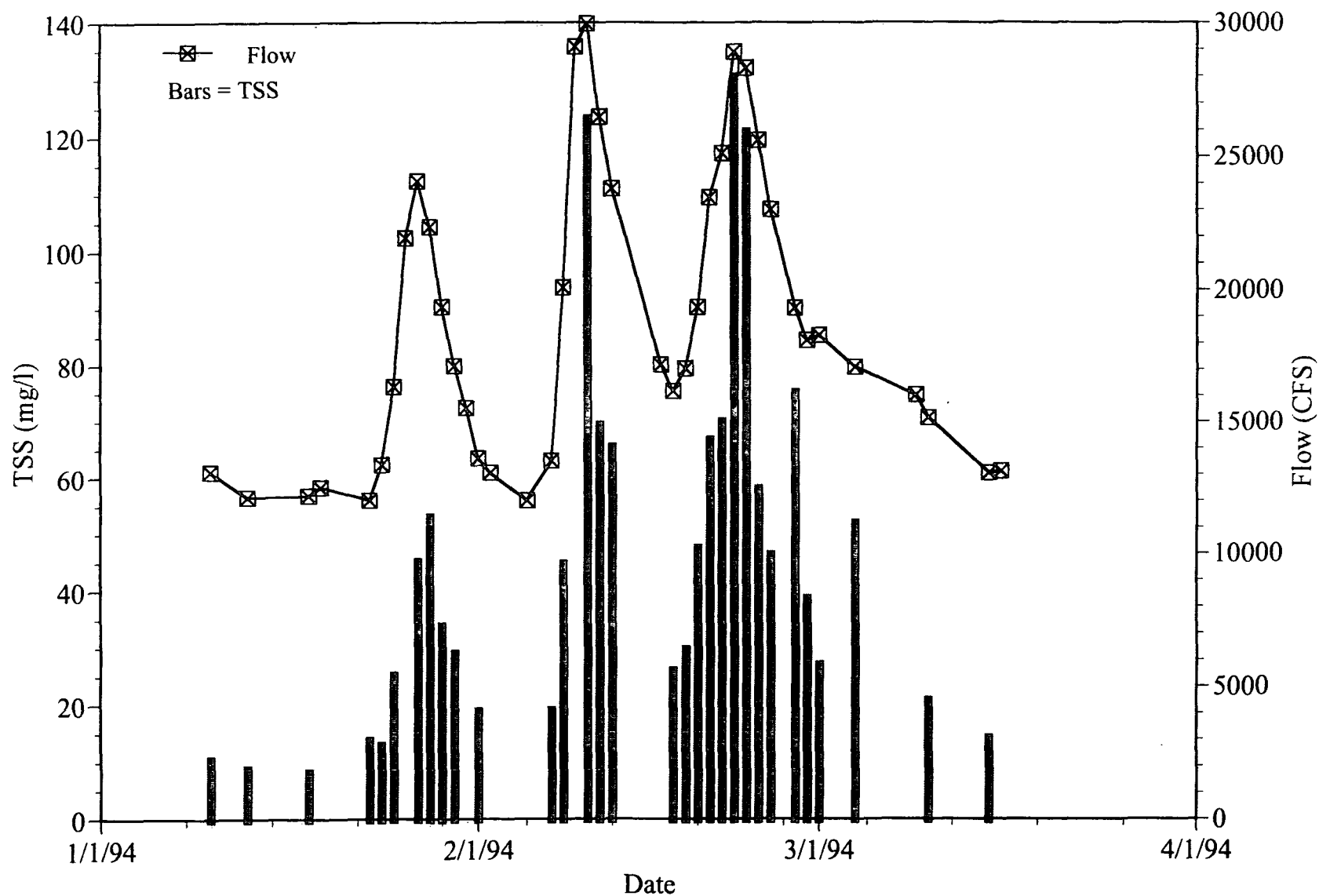
Figure 66. Flow and total suspended solids (TSS) pattern in the Sacramento River at Greene's Landing during low flow conditions from January through March of 1994.
