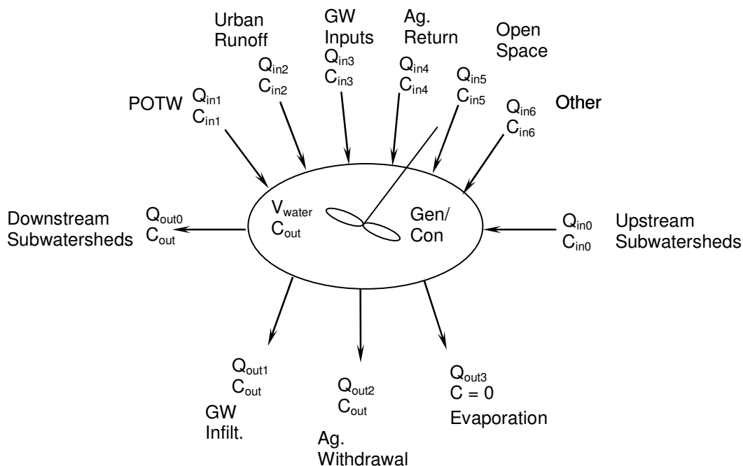
Figure 21: Schematic of Inputs and Outputs for a General Computational Element used in the CCMS Mass Balance Model to Estimate Water Flow and Quality within Surface Water Reaches.
