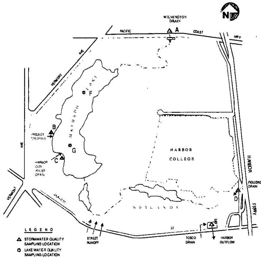
Figure 2-5 Current Water Quality Sampling Locations at Machado Lake
