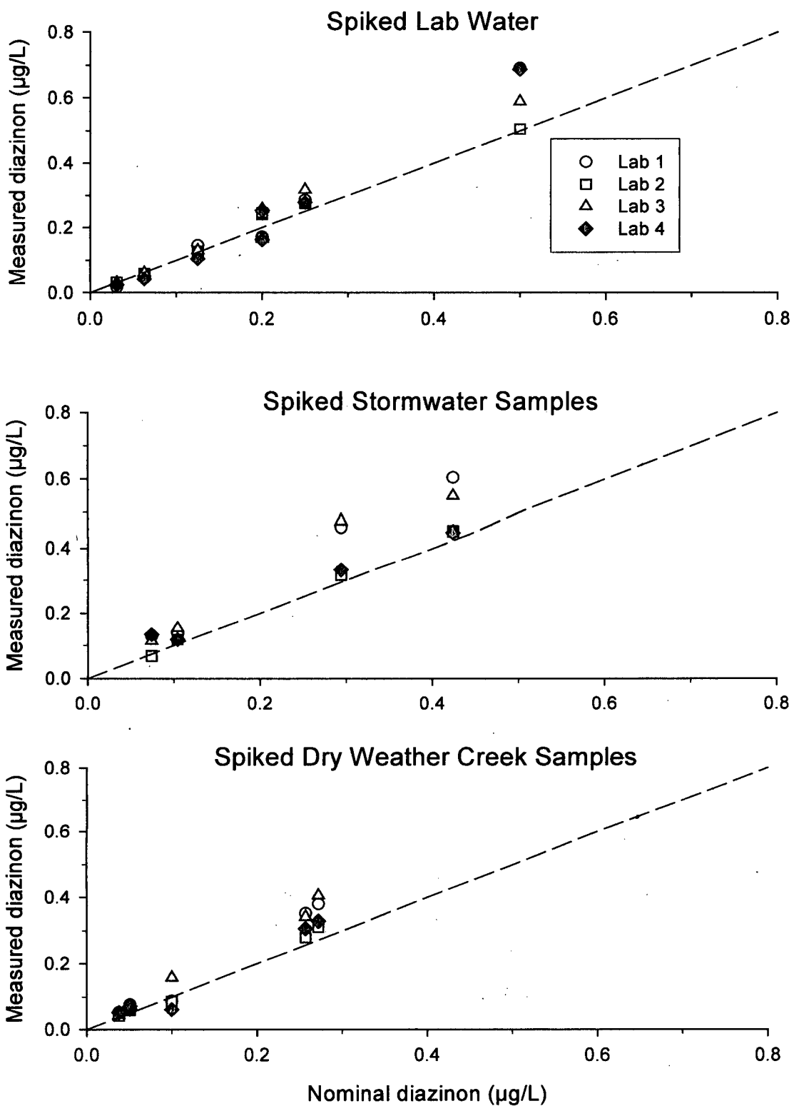
Figure 9. Measured vs nominal concentrations of diazinon associated with spiked lab water, storm water, and dry weather runoff during the ELISA interlab comparison. The dashed line represents the theoretical one-to-one relationship between measured and nominal concentrations.
