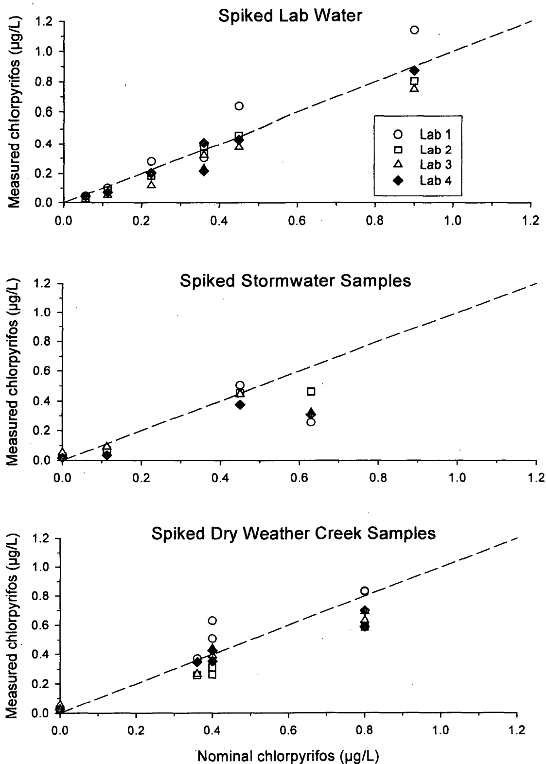
Figure 10. Measured vs nominal concentrations of chlorpyrifos associated with spiked lab water, storm water, and dry weather runoff during the ELISA interlab comparison. The dashed line represents the theoretical one-to-one relationship between measured and nominal concentrations.
