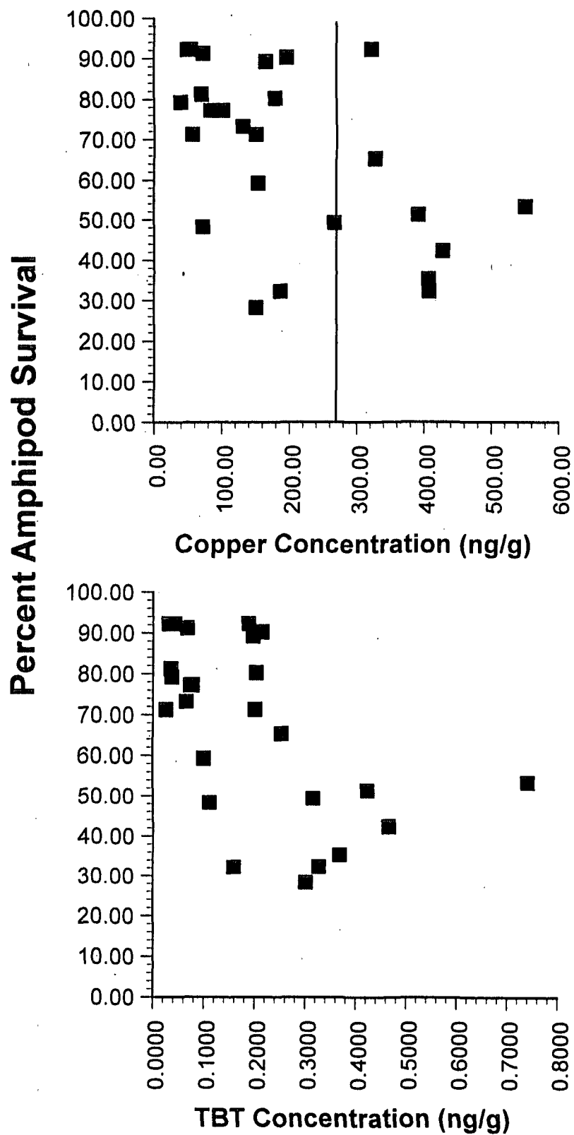
Figure 50. Amphipod survival at Marina stations in relation to copper and TBT concentrations. Vertical line indicates ERM value for copper.
