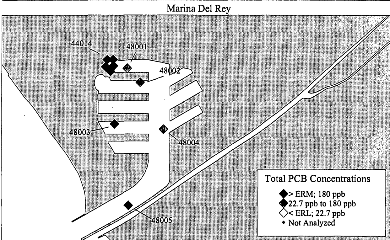
Figures 42a and 42b. Distribution of samples in King Harbor (a), and Marina Del Rey (b), exceeding the ERM for Total PCB.
