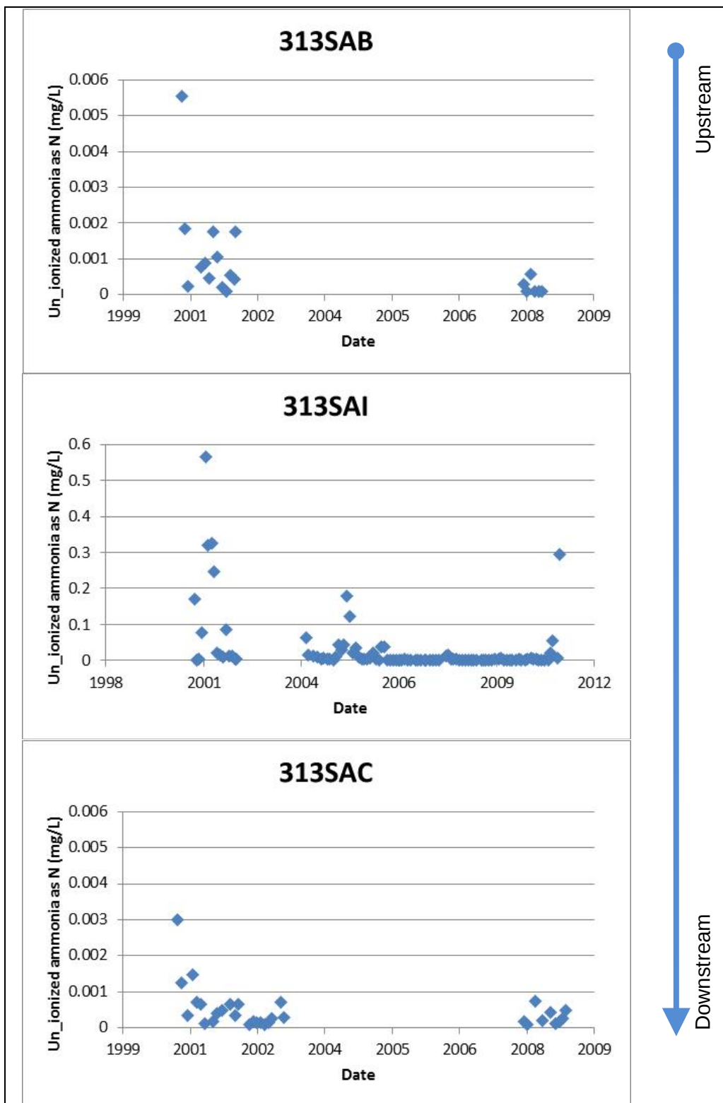
Figure 4-4. Scatter plots of un-ionized ammonia as nitrogen (mg/L) concentrations. Note that the water quality objective for un-ionized ammonia is 0.025 mg/L as nitrogen and that the vertical axis is different for site 313SAI due to higher maximum values.
