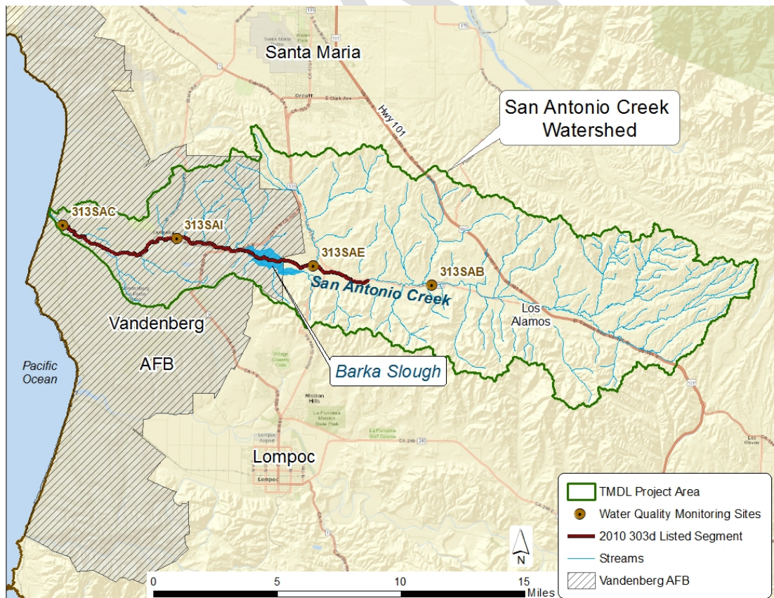
Figure 1-2. San Antonio Creek 2008-2010 303(d)-Listed segment and CCAMP monitoring sites.
