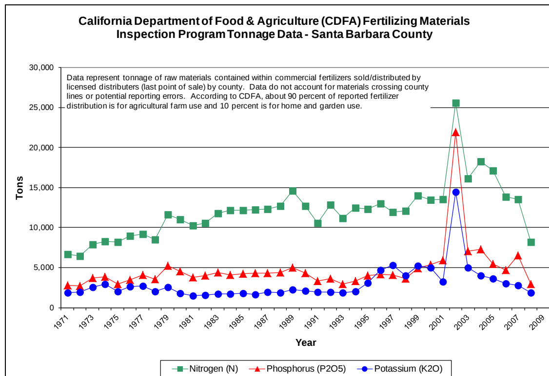
Figure 6-2. Fertilizer sales in Santa Barbara County.
