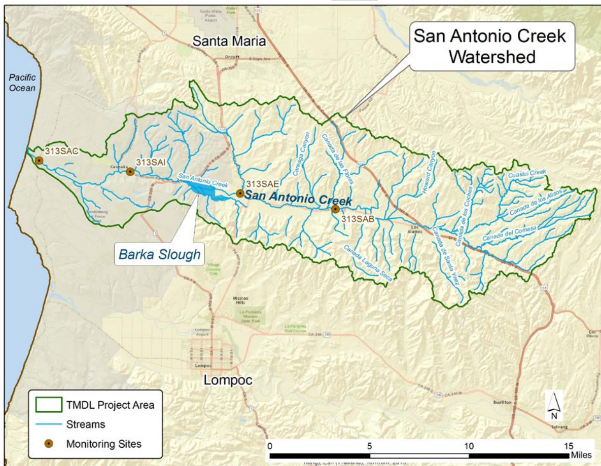
Figure 2-1. Streams and CCAMP monitoring sites.
