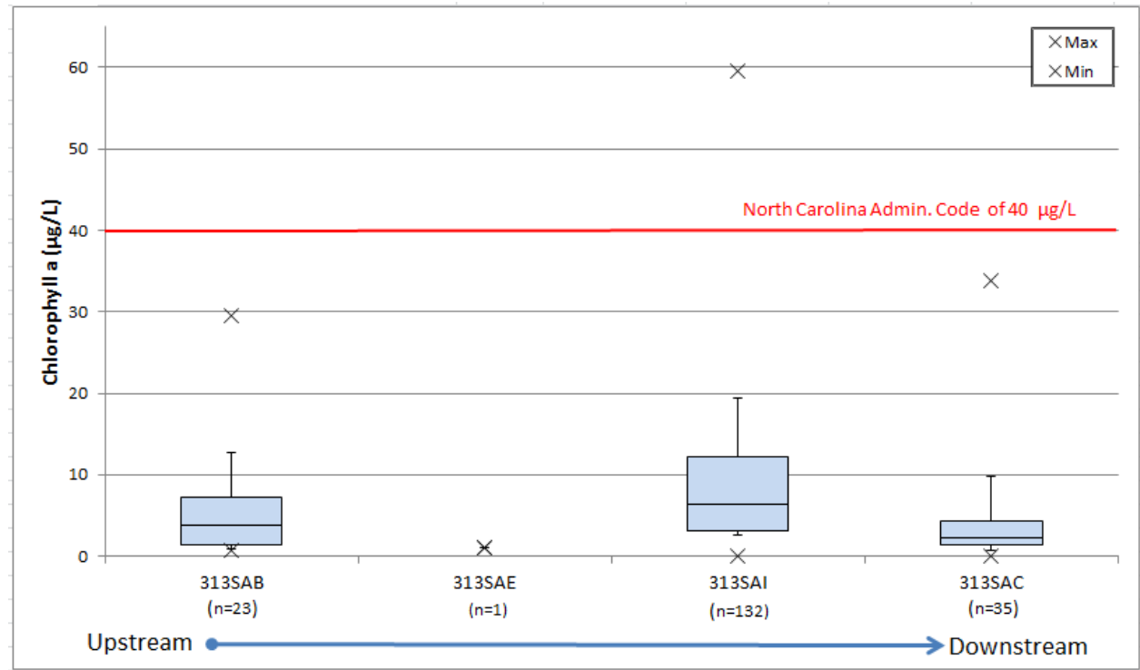
Figure 4-16. Boxplots of chlorophyll a (µg/L) concentrations.
