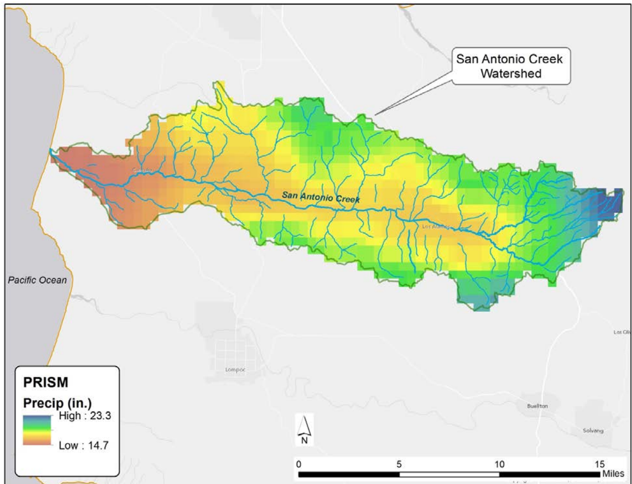
Figure 2-6. Average annual precipitation 1971-2000. Source: PRISM Climate Group, Oregon State University
