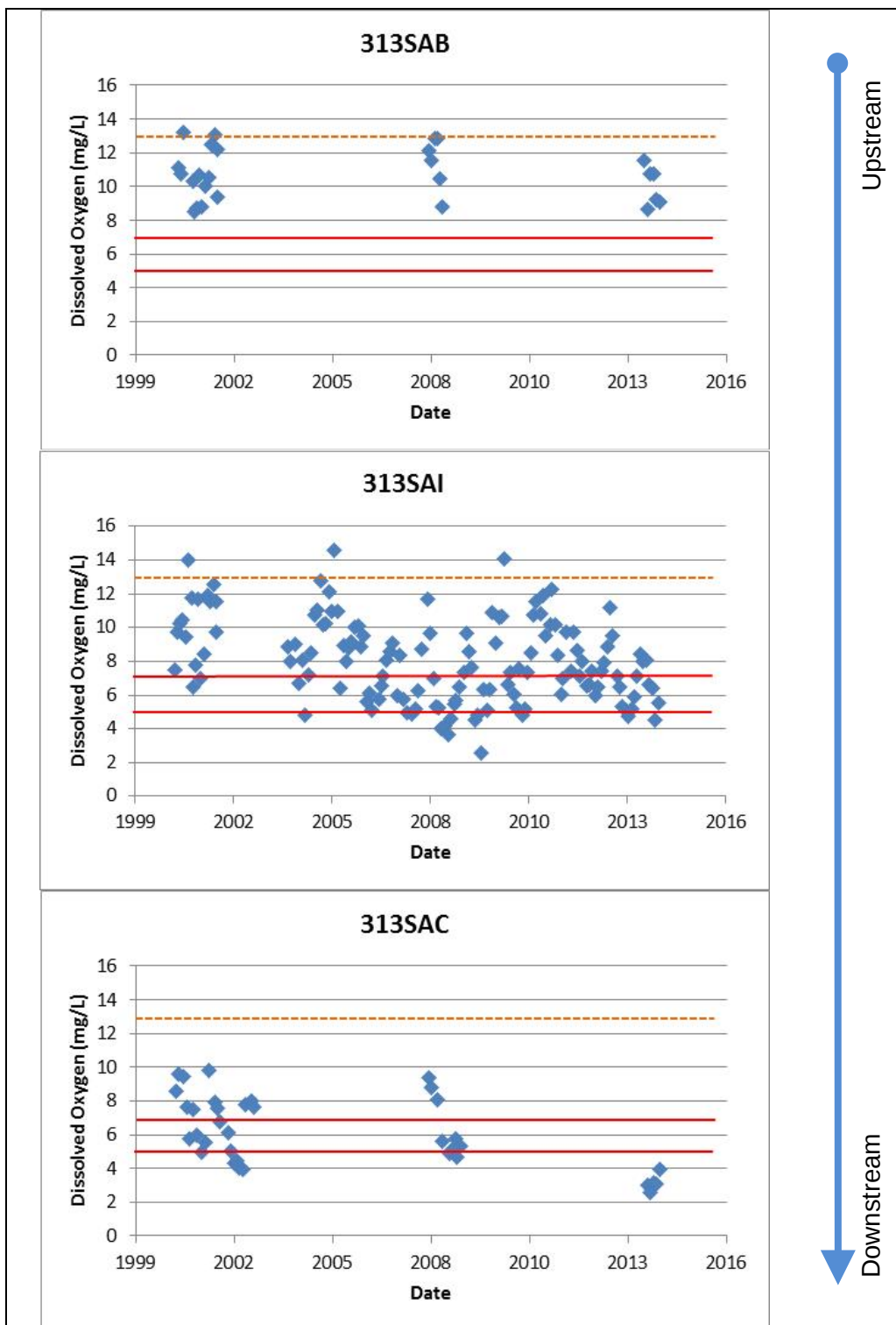
Figure 4-12. Scatter plot of dissolved oxygen concentrations (mg/L).
