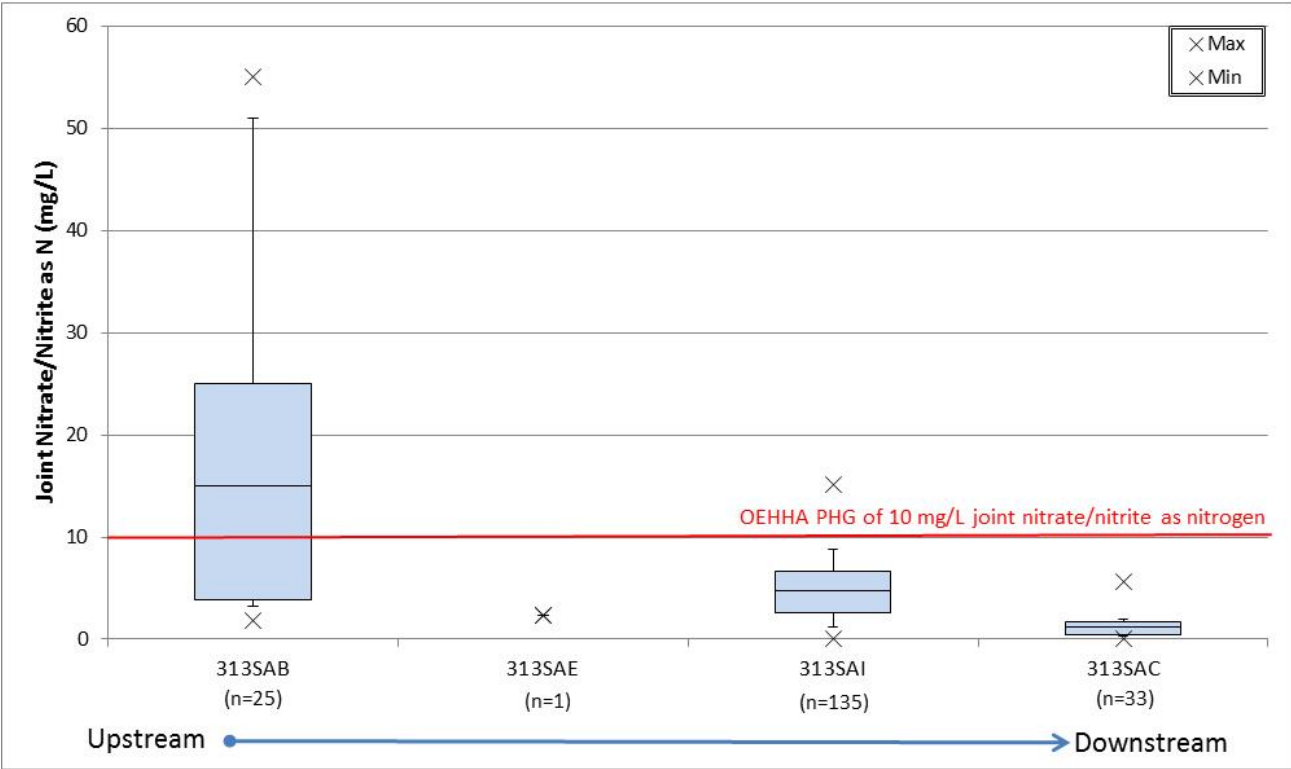
Figure 4-9. Box plots of joint nitrate/nitrite as nitrogen (mg/L) concentrations.
