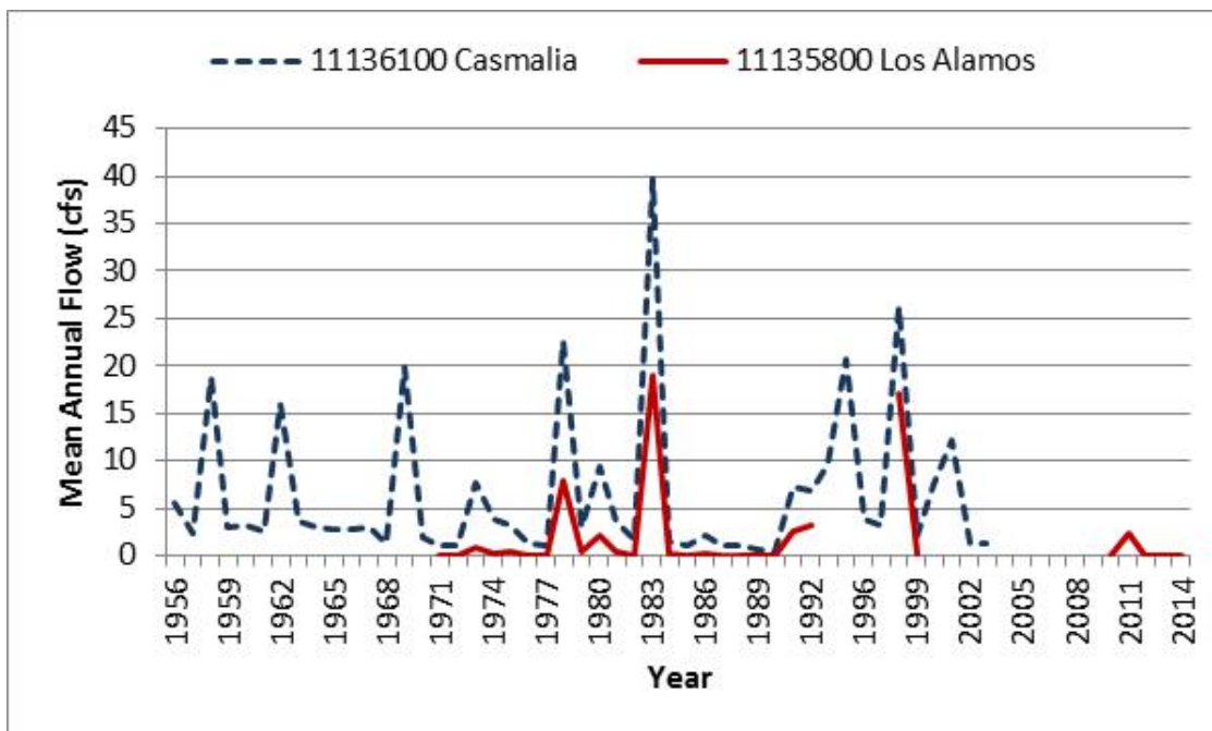
Figure 2-4. USGS mean annual flow.
