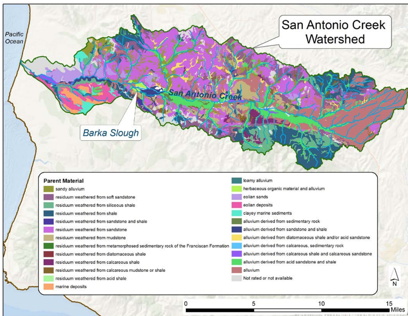
Figure C-8. SSURGO Parent Material
