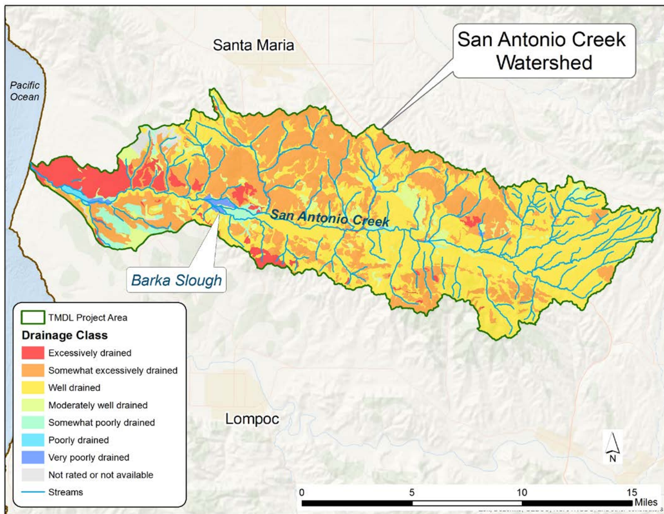
Figure C-7. SSURGO Drainage Class
