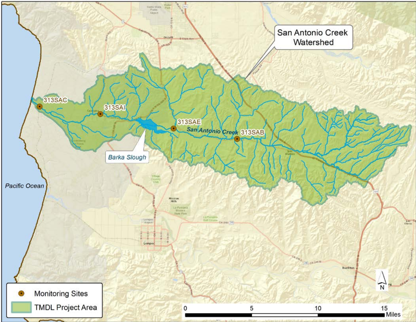
Figure 4-1 Location of CCAMP water quality monitoring stations.
