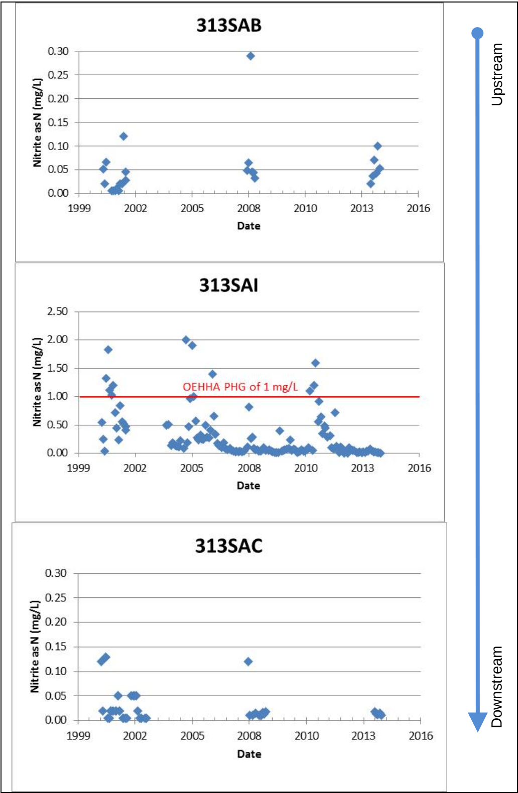
Figure 4-6. Scatter plot of nitrite as nitrogen concentrations (mg/L). Note that the vertical axis is different for site 313SAI due to higher maximum values
