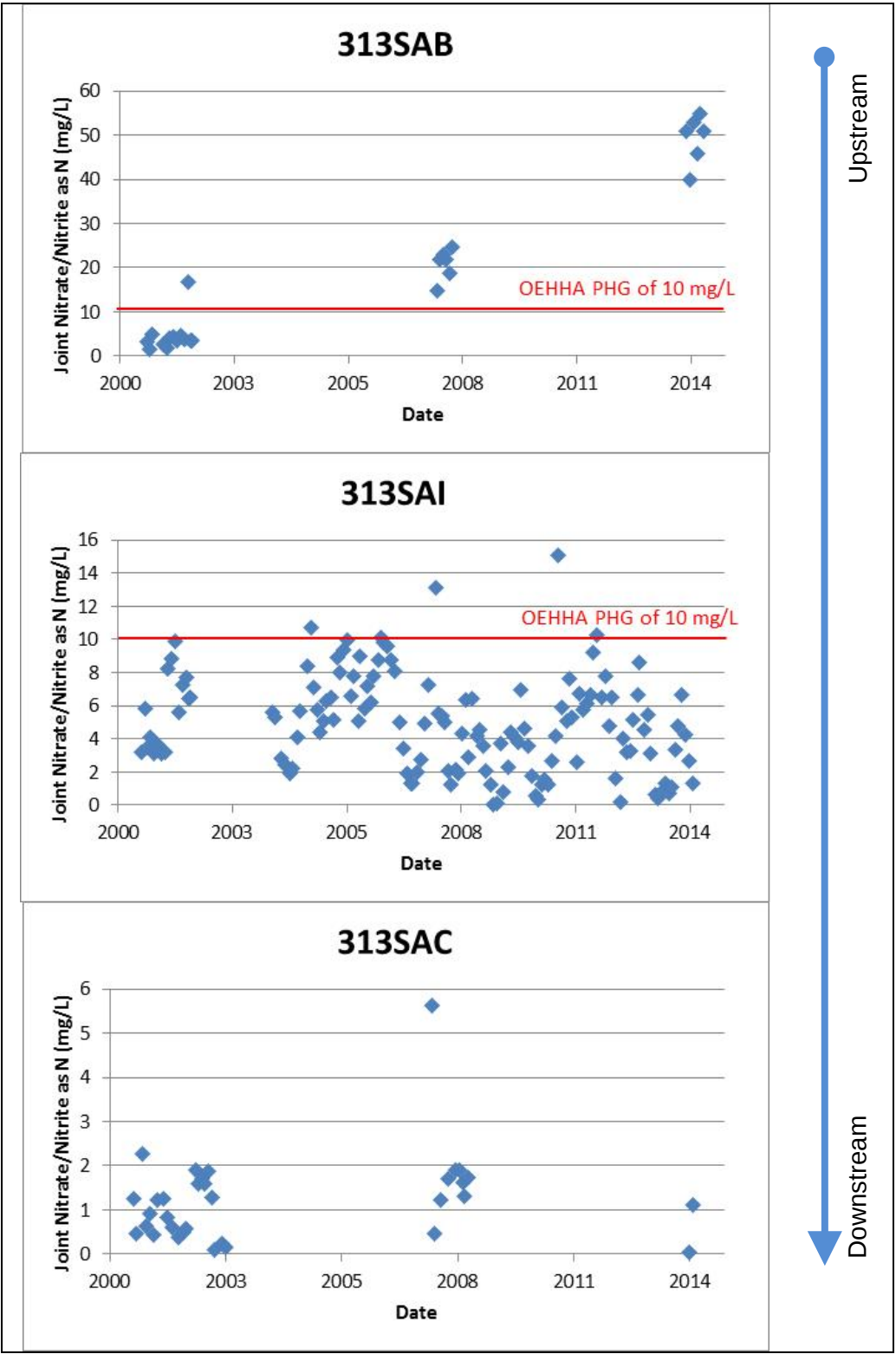
Figure 4-10. Scatter plot of joint nitrate/nitrite as nitrogen concentrations. Note that the vertical axis is different for each site.
