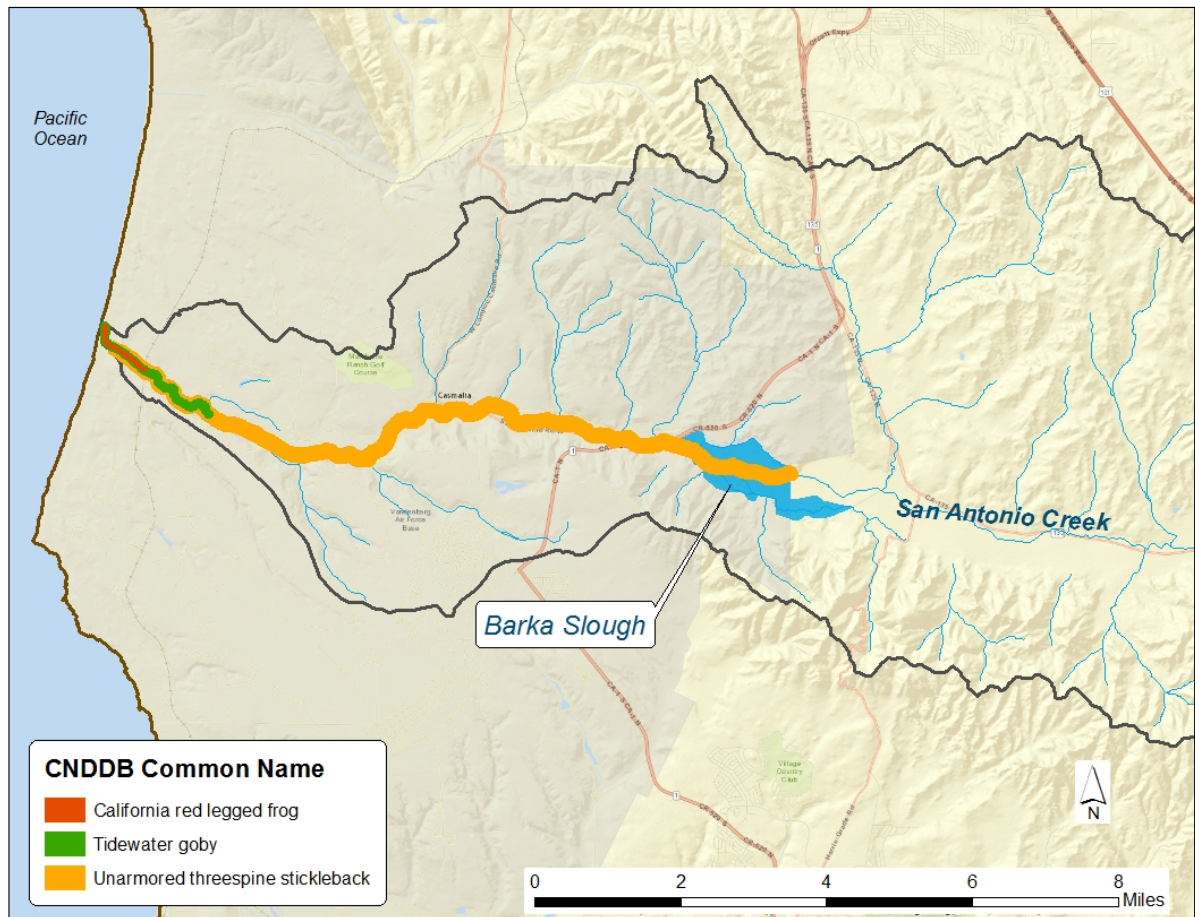
Figure 2-7. Location of sensitive aquatic species and habitat.
