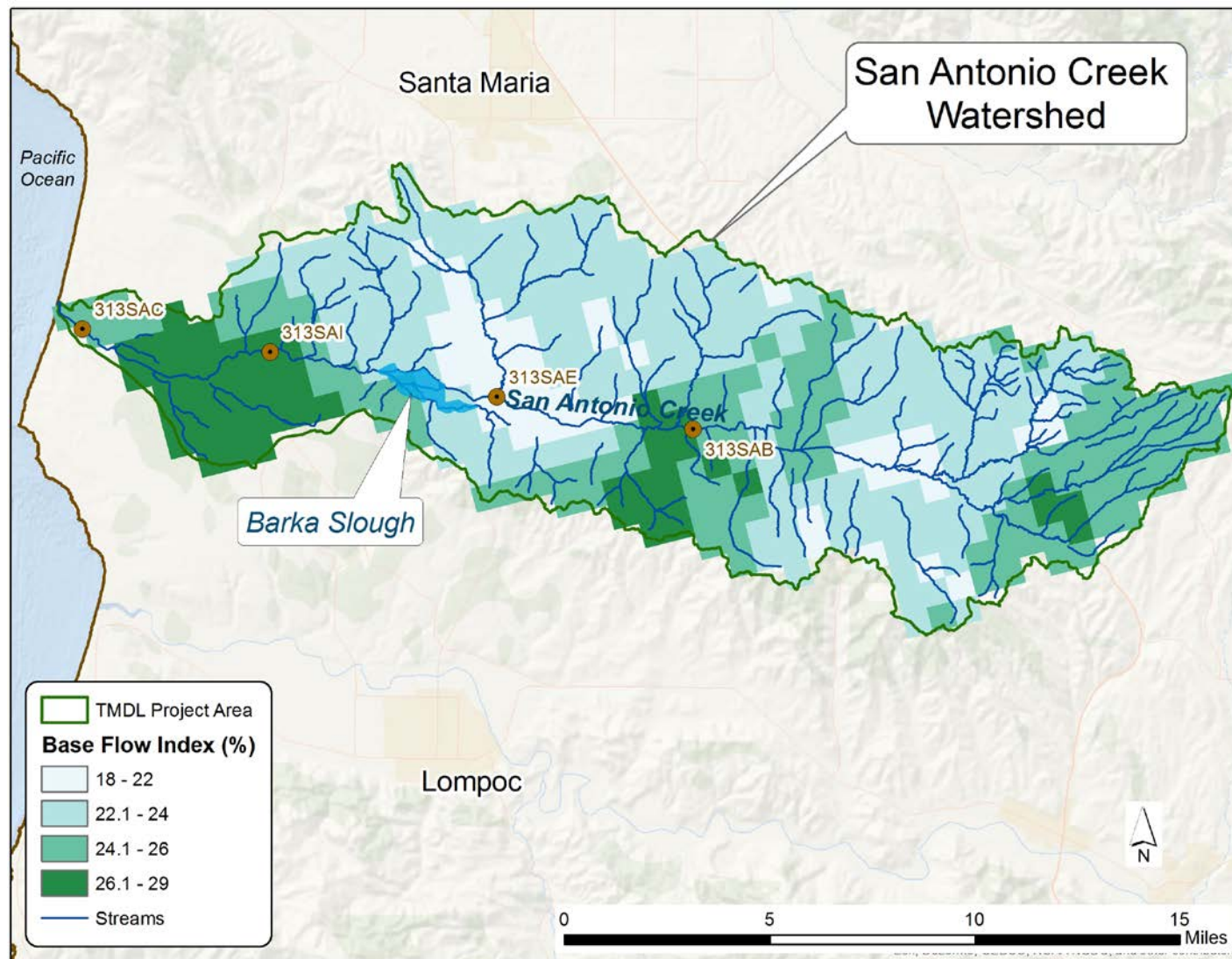
Figure C-1. Base-flow Index (%).
