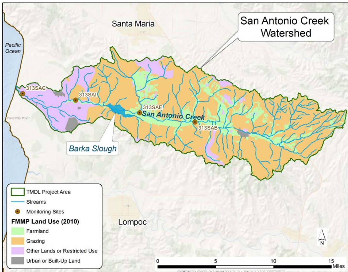
Figure 2-3. Land use and CCAMP monitoring sites.
