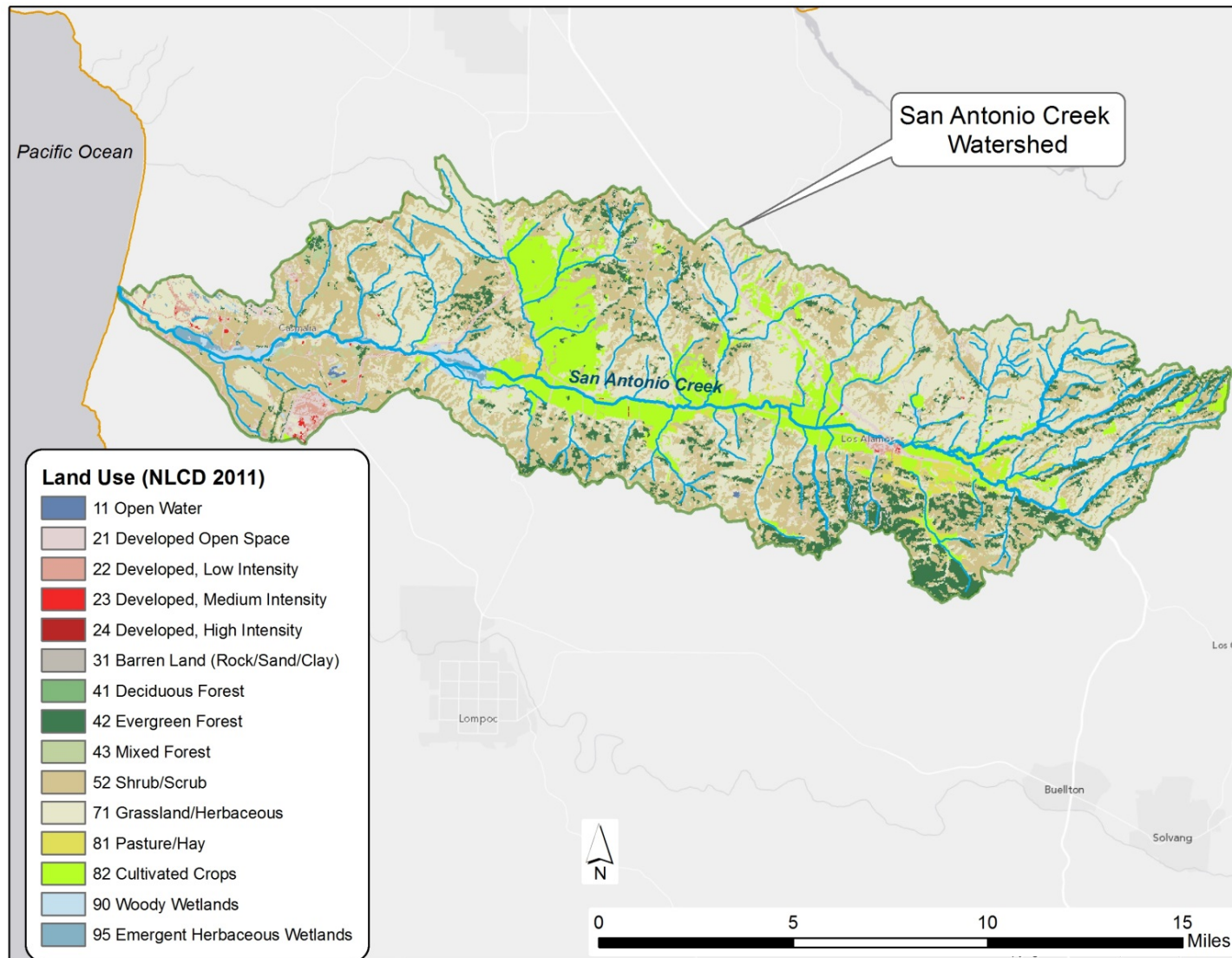
Figure C-2. NLCD land use
