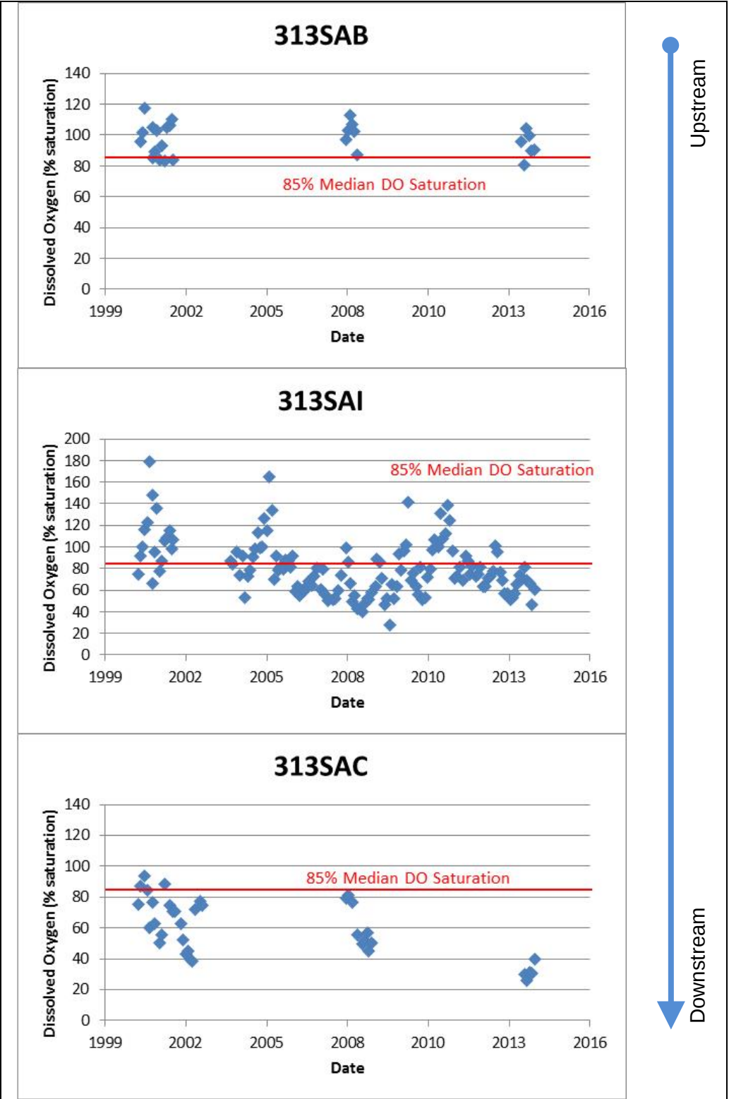
Figure 4-14. Scatter plot of dissolved oxygen saturation (%).
