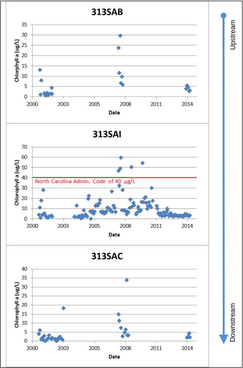
Figure 4-17. Scatter plot of chlorophyll a concentrations (µg/L).
