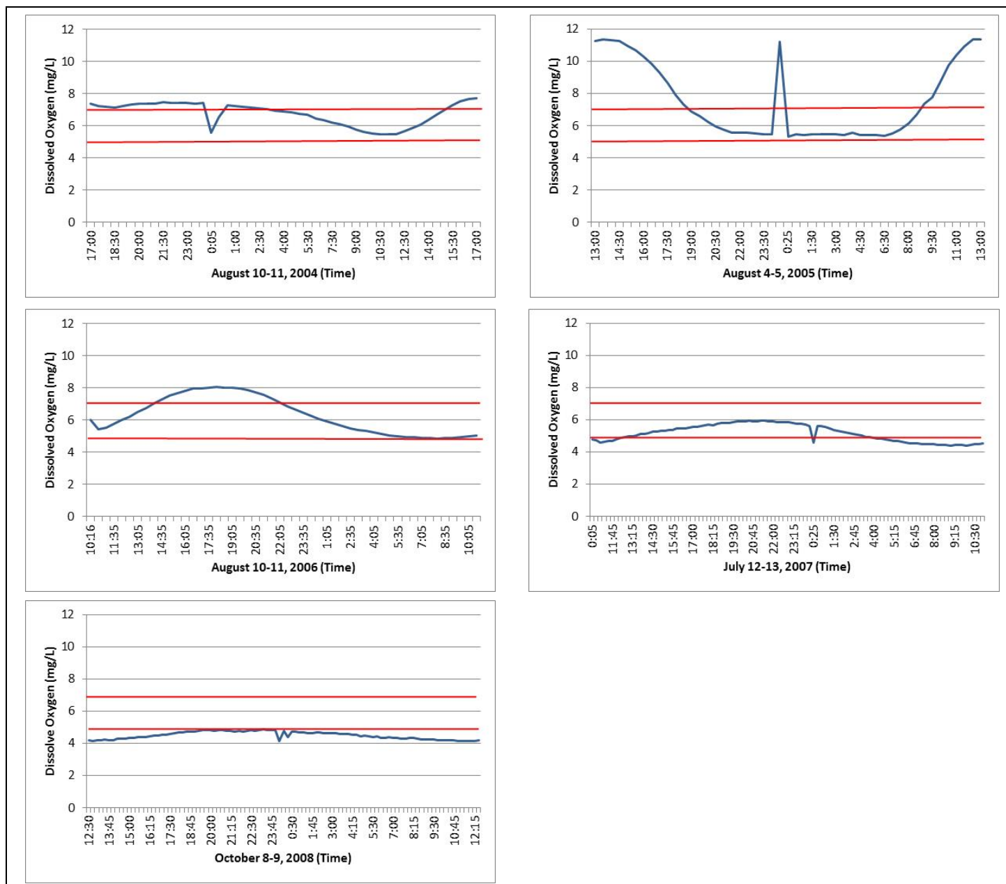
Figure 4-15. CCAMP diel dissolved oxygen concentrations (mg/L) for site 313SAI (2004-2008).
