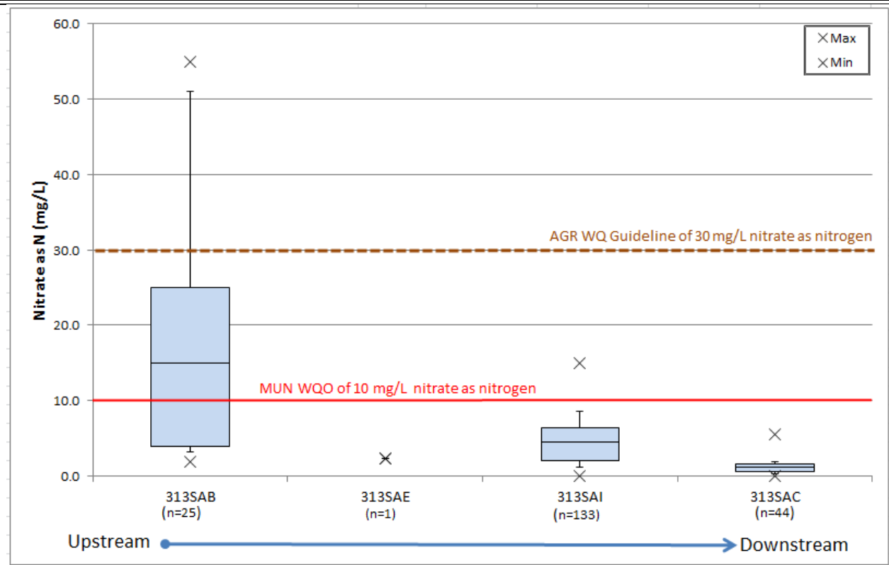
Figure 4-7. Box plots of nitrate as nitrogen (mg/L) concentrations.
