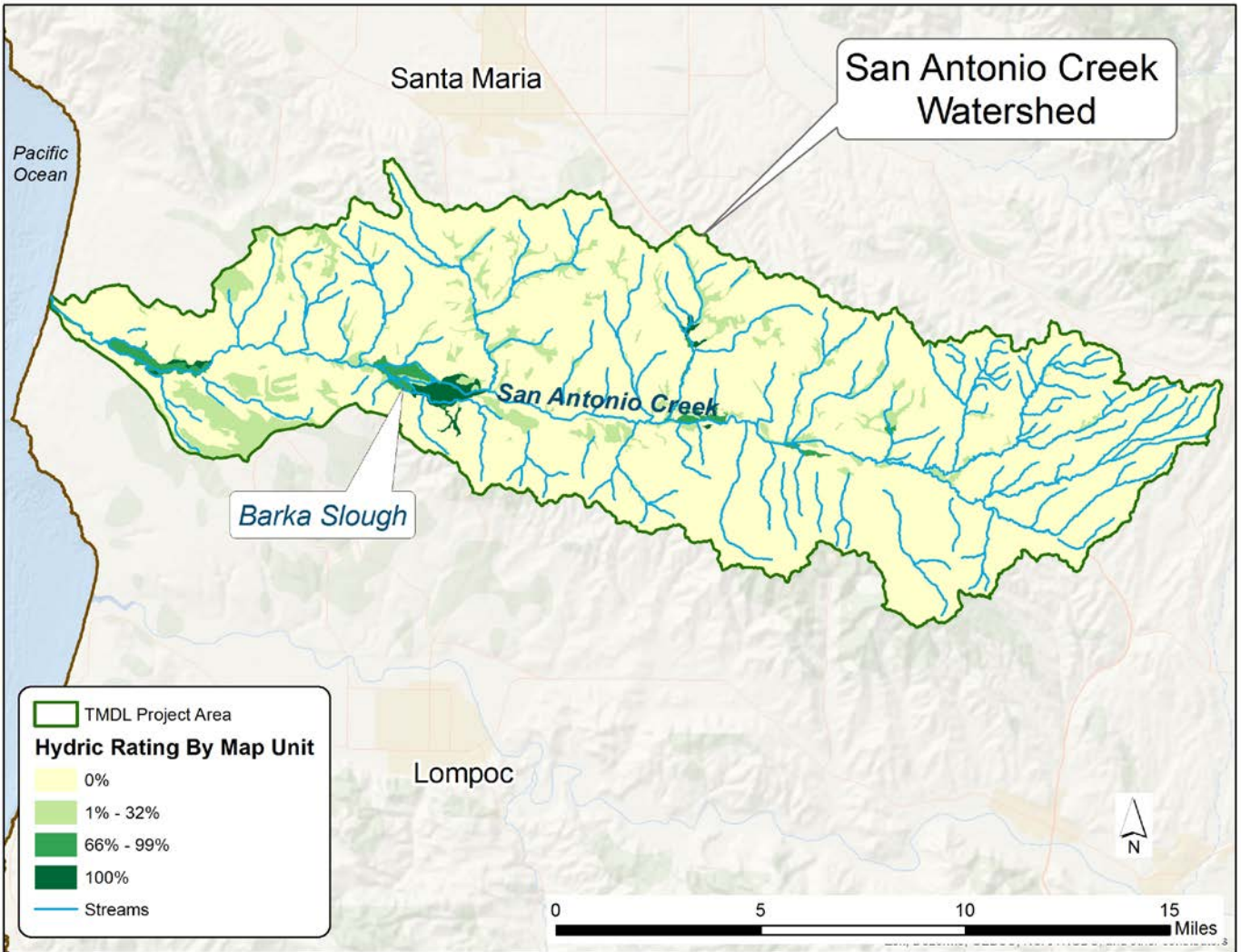
Figure C-5. SSURGO Hydric Rating
