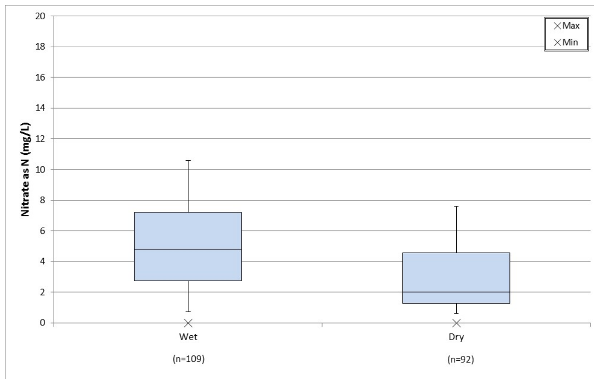
Figure 7-1. Wet season (Nov-Apr) and dry season (May-Oct) plots. Not shown: Wet and dry maximum values of 53 mg/L and 55 mg/L, respectively.
