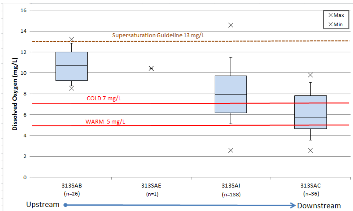
Figure 4-11. Boxplots of dissolved oxygen concentrations (mg/L).
