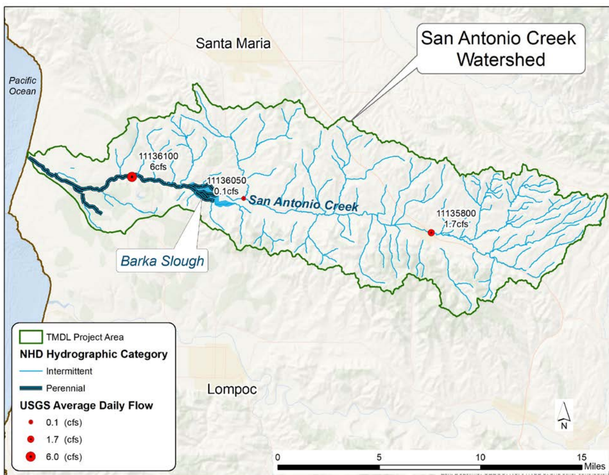
Figure 2-5. USGS gage locations, stream flow characteristics, and stream types. Spatial data sources: USGS National Hydrography Dataset (NHD), High Resolution (1:24,000) representing hydrographic category. USGS average daily flow based on streamflow characteristics dataset (Wolock, 2003) containing data up through November 2001.
