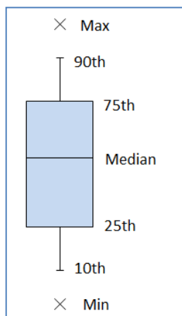
Figure 4-2. Explanation of box plots.
