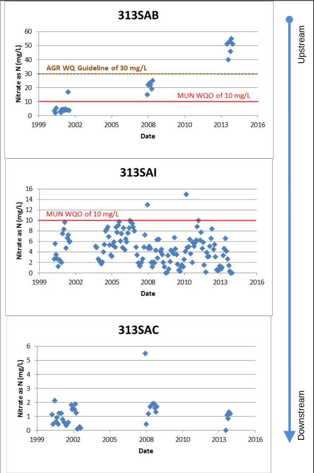
Figure 4-8. Scatter plot of nitrate as nitrogen concentrations (mg/L). Note that the vertical axis is different for each site.
