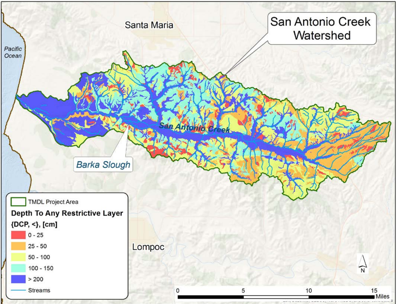
Figure C-10. SSURGO Depth to Any Restrictive Layer
