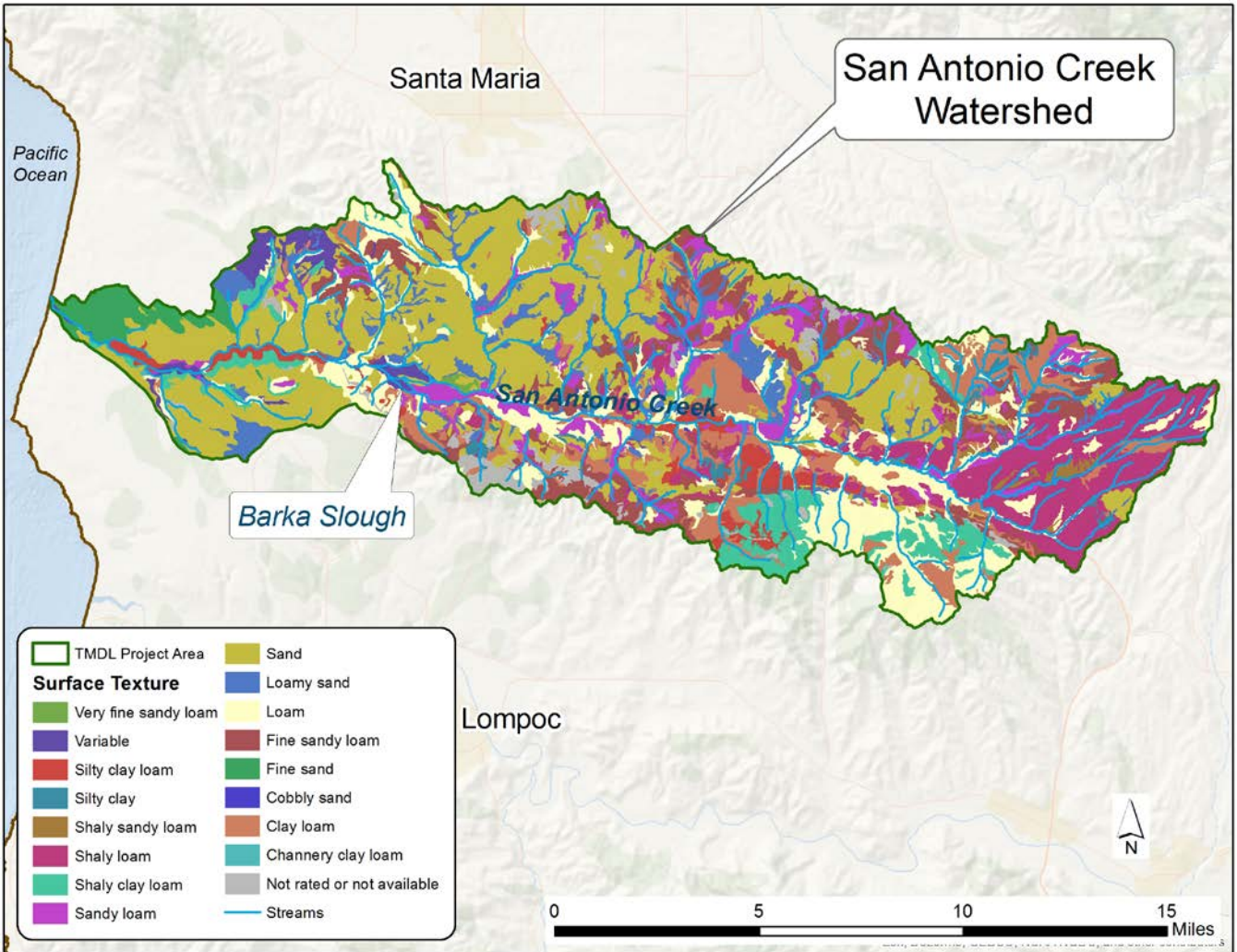
Figure C-6. SSURGO Surface Texture
