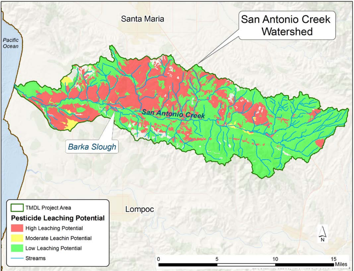
Figure C-4. SSURGO Pesticide Leaching Potential
