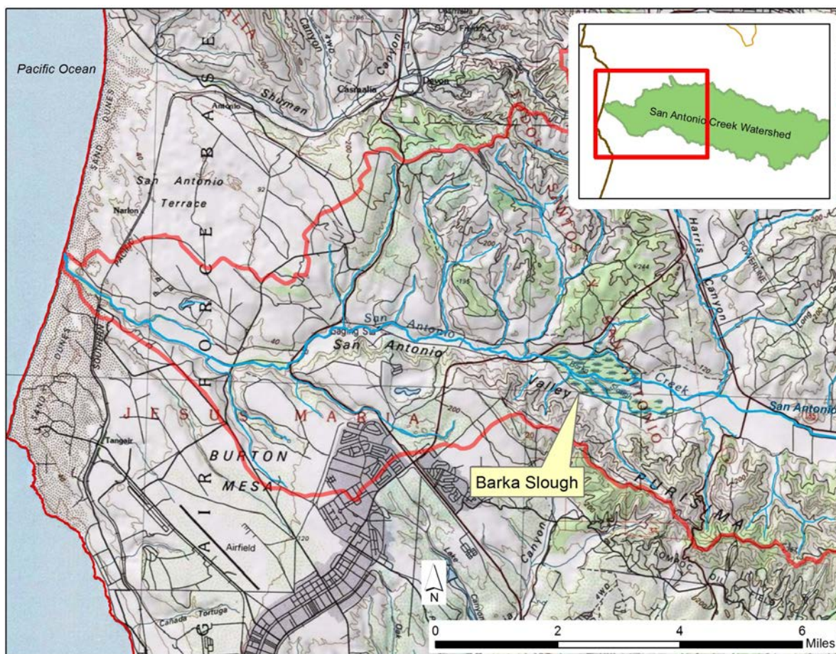
Figure 2-2. Location of Barka Slough.
