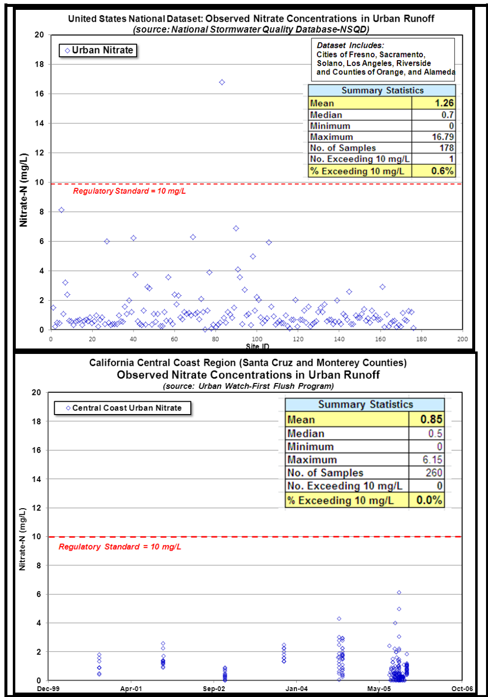
Figure 6-1. Nitrate concentration in urban runoff: national, California, and central coast regional data.
