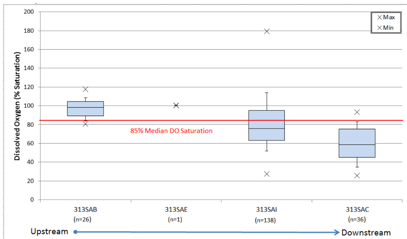
Figure 4-13. Boxplots of dissolved oxygen saturation (%).
