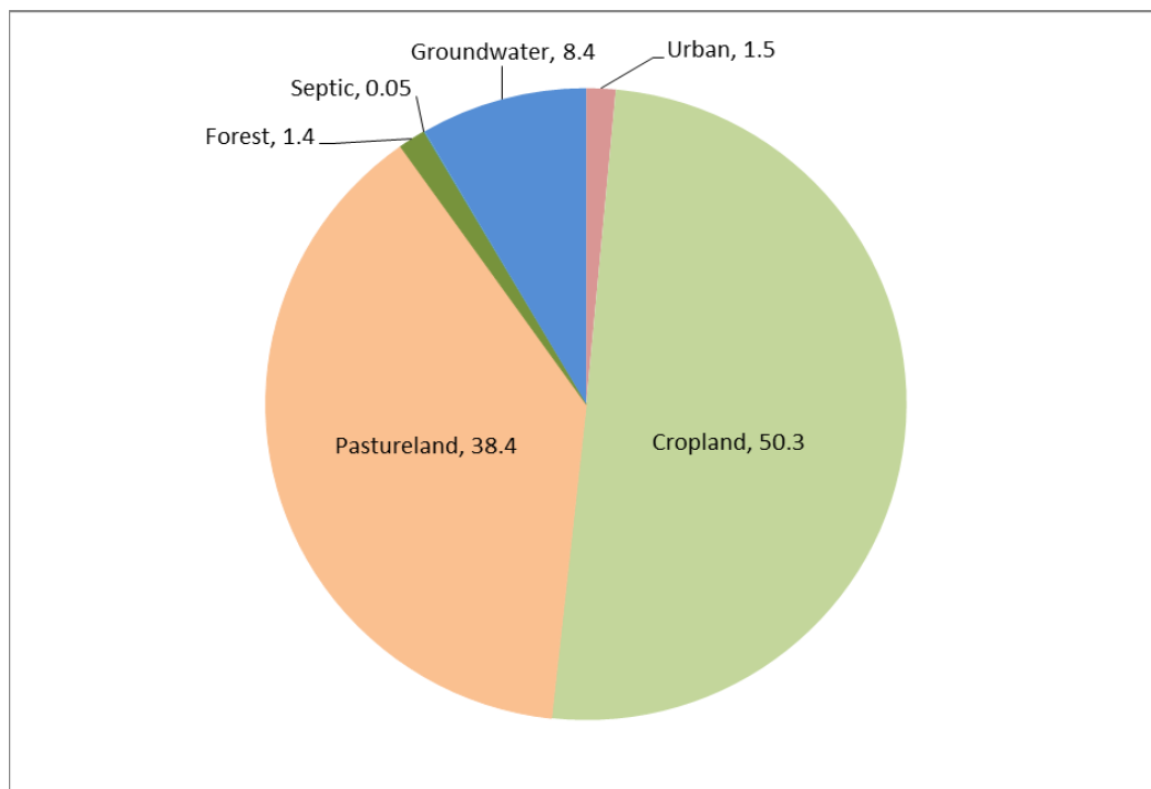
Figure 6-3. Summary of estimated nitrate loads (%).
