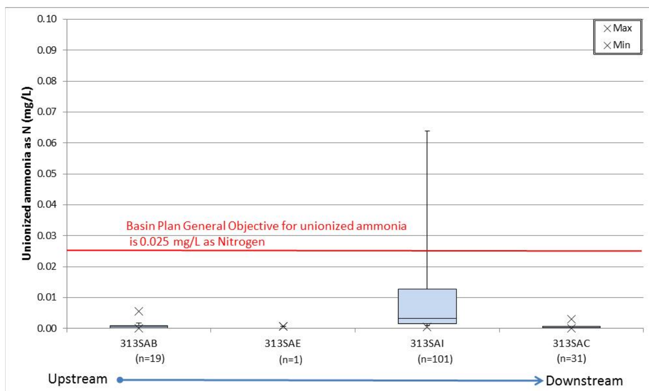
Figure 4-3. Box plots of un-ionized ammonia as nitrogen (mg/L) concentrations.
