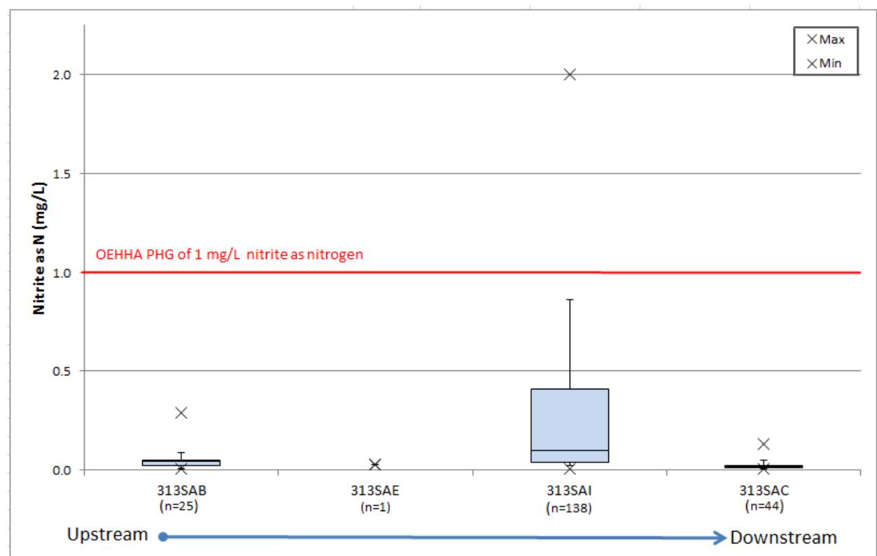
Figure 4-5. Box plots of nitrite as nitrogen (mg/L) concentrations.
