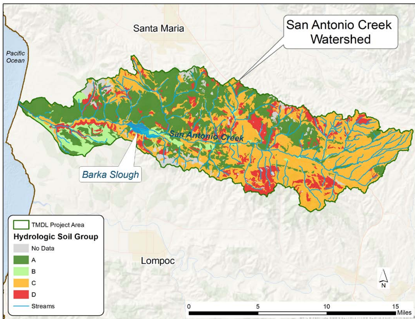
Figure C-9. SSURGO Hydrologic Soil Group
