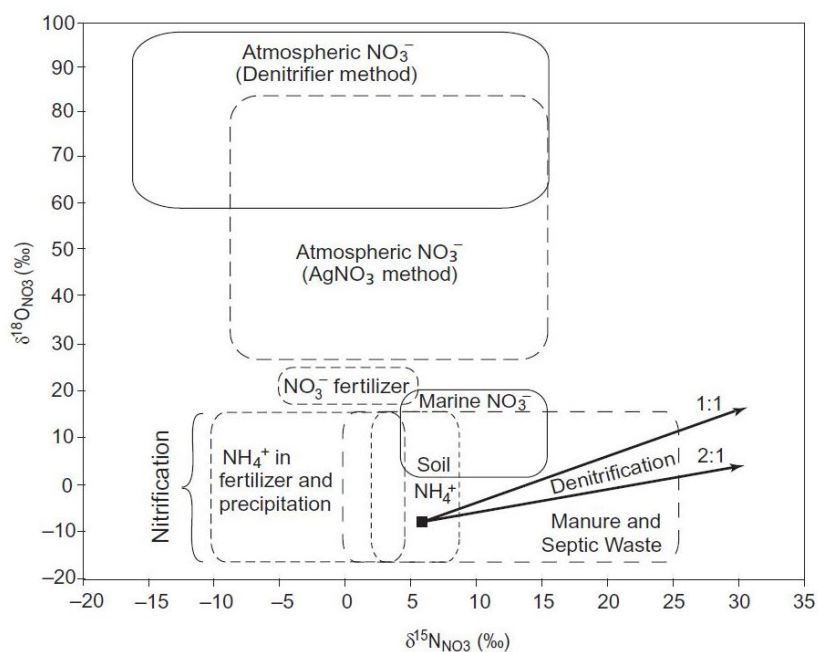
Figure 22. Typical values of the Stable Isotopes of oxygen ( \delta^{18}\text{O} ) and nitrogen ( \delta^{15}\text{N} ) of nitrate derived from various sources (diagram from Michener and Lajtha, 2007).
